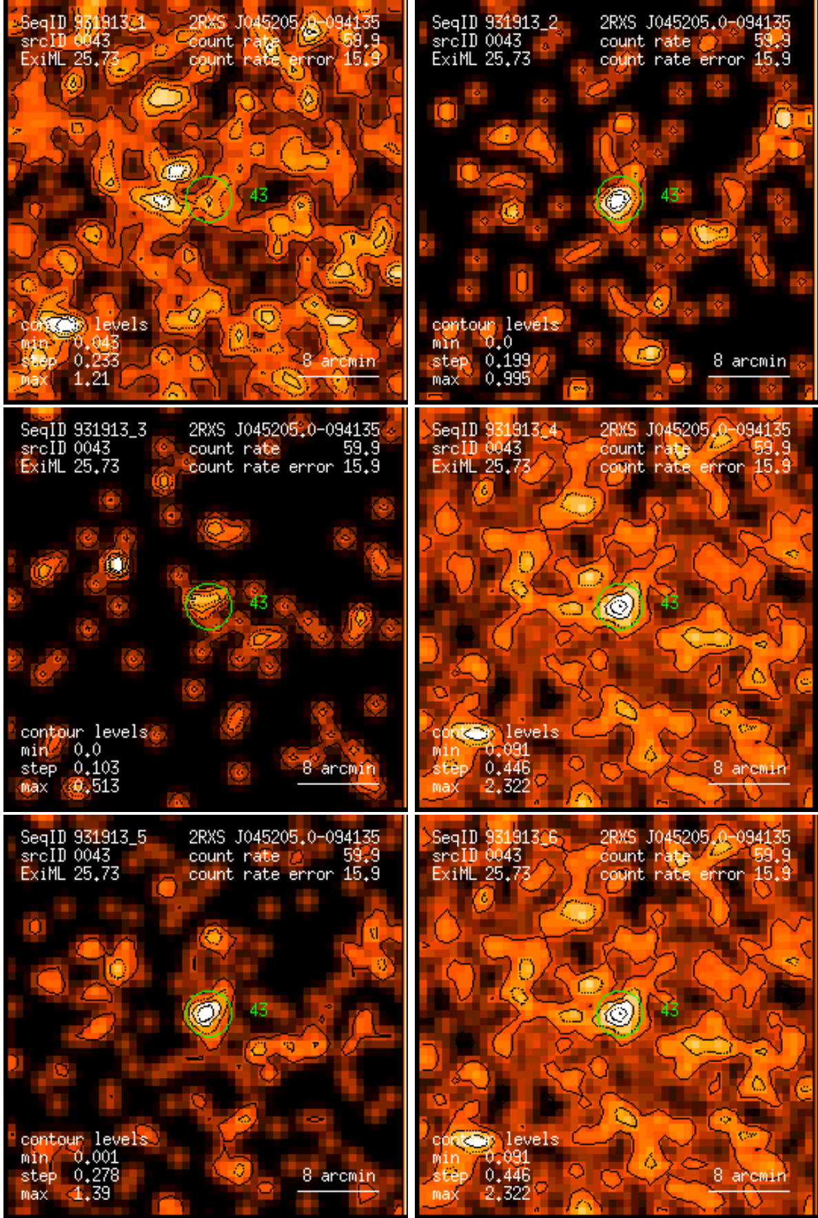
Figure 43: RASS 931913: detection 0043: band rate images, Gaussian filter: (1) PSPC channels 11 – 41, (2) 52 – 90, (3) 91 – 201, (4) 11 – 235, (5) 52 – 201, (6) 11 – 201. Broad band rates in counts/ks. Band rate contour levels in counts/ks/arcmin 2 .
