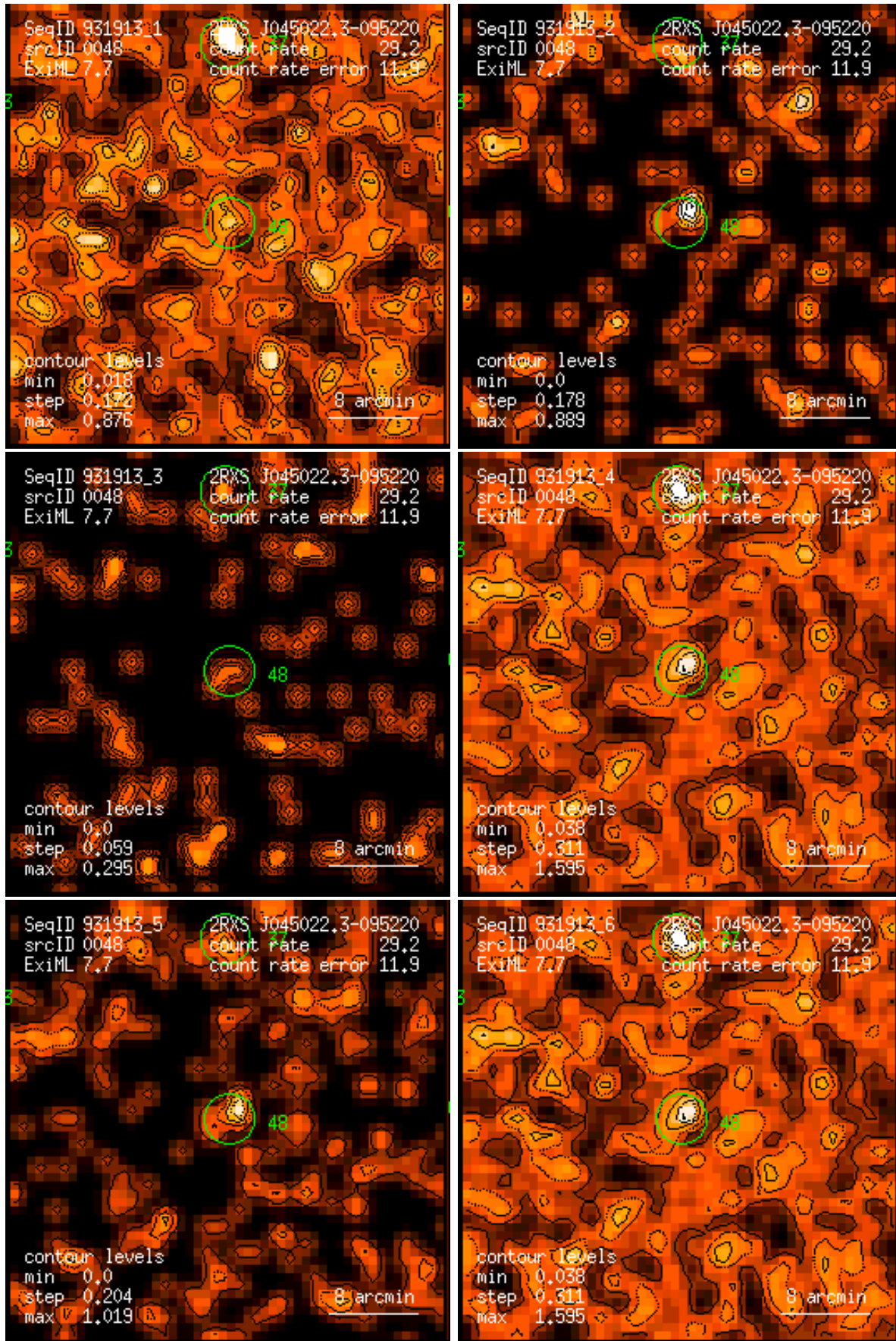
Figure 48: RASS 931913: detection 0048: band rate images, Gaussian filter: (1) PSPC channels 11 – 41, (2) 52 – 90, (3) 91 – 201, (4) 11 – 235, (5) 52 – 201, (6) 11 – 201. Broad band rates in counts/ks. Band rate contour levels in counts/ks/arcmin 2 .
