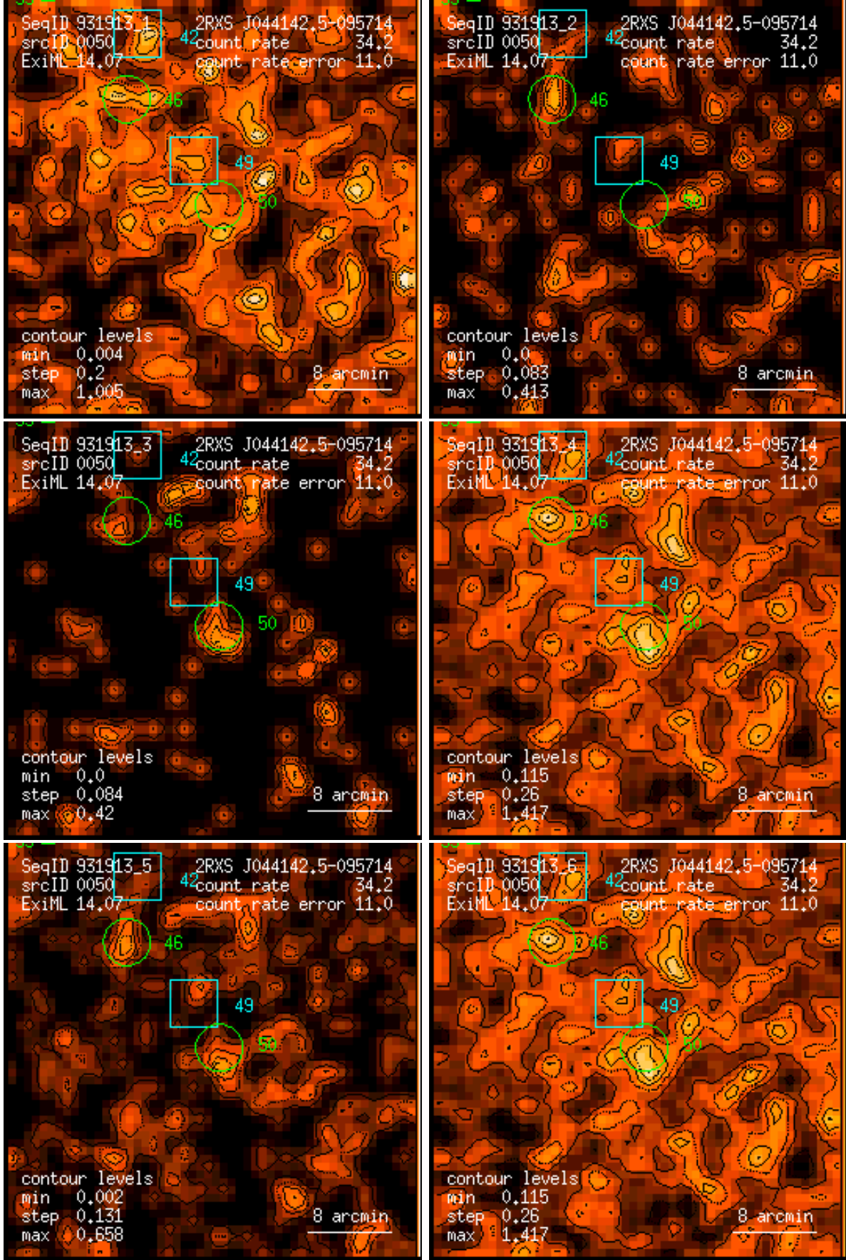
Figure 50: RASS 931913: detection 0050: band rate images, Gaussian filter: (1) PSPC channels 11 – 41, (2) 52 – 90, (3) 91 – 201, (4) 11 – 235, (5) 52 – 201, (6) 11 – 201. Broad band rates in counts/ks. Band rate contour levels in counts/ks/arcmin 2 .
