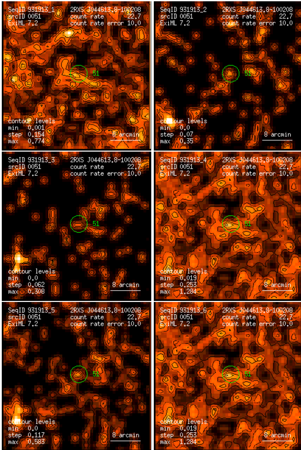
Figure 51: RASS 931913: detection 0051: band rate images, Gaussian filter: (1) PSPC channels 11 – 41, (2) 52 – 90, (3) 91 – 201, (4) 11 – 235, (5) 52 – 201, (6) 11 – 201. Broad band rates in counts/ks. Band rate contour levels in counts/ks/arcmin 2 .
