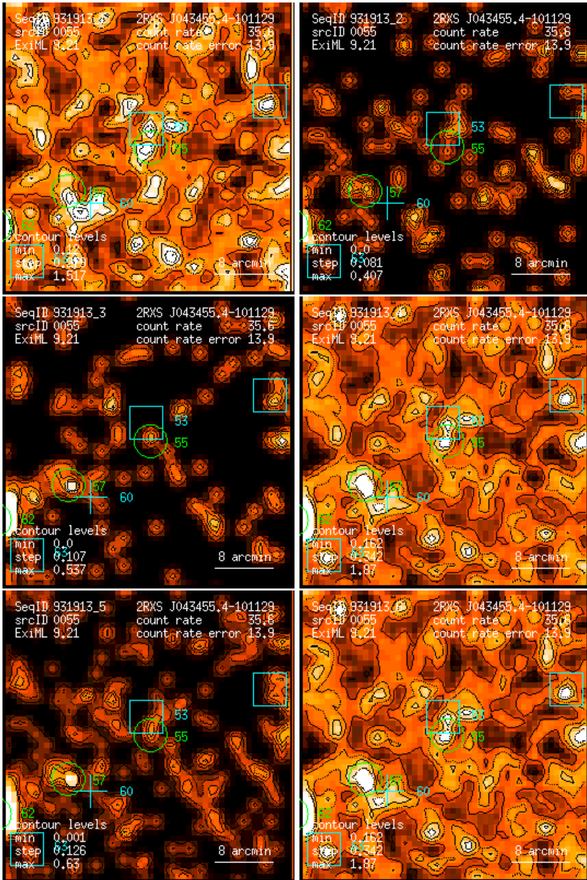
Figure 55: RASS 931913: detection 0055: band rate images, Gaussian filter: (1) PSPC channels 11 – 41, (2) 52 – 90, (3) 91 – 201, (4) 11 – 235, (5) 52 – 201, (6) 11 – 201. Broad band rates in counts/ks. Band rate contour levels in counts/ks/arcmin 2 .
