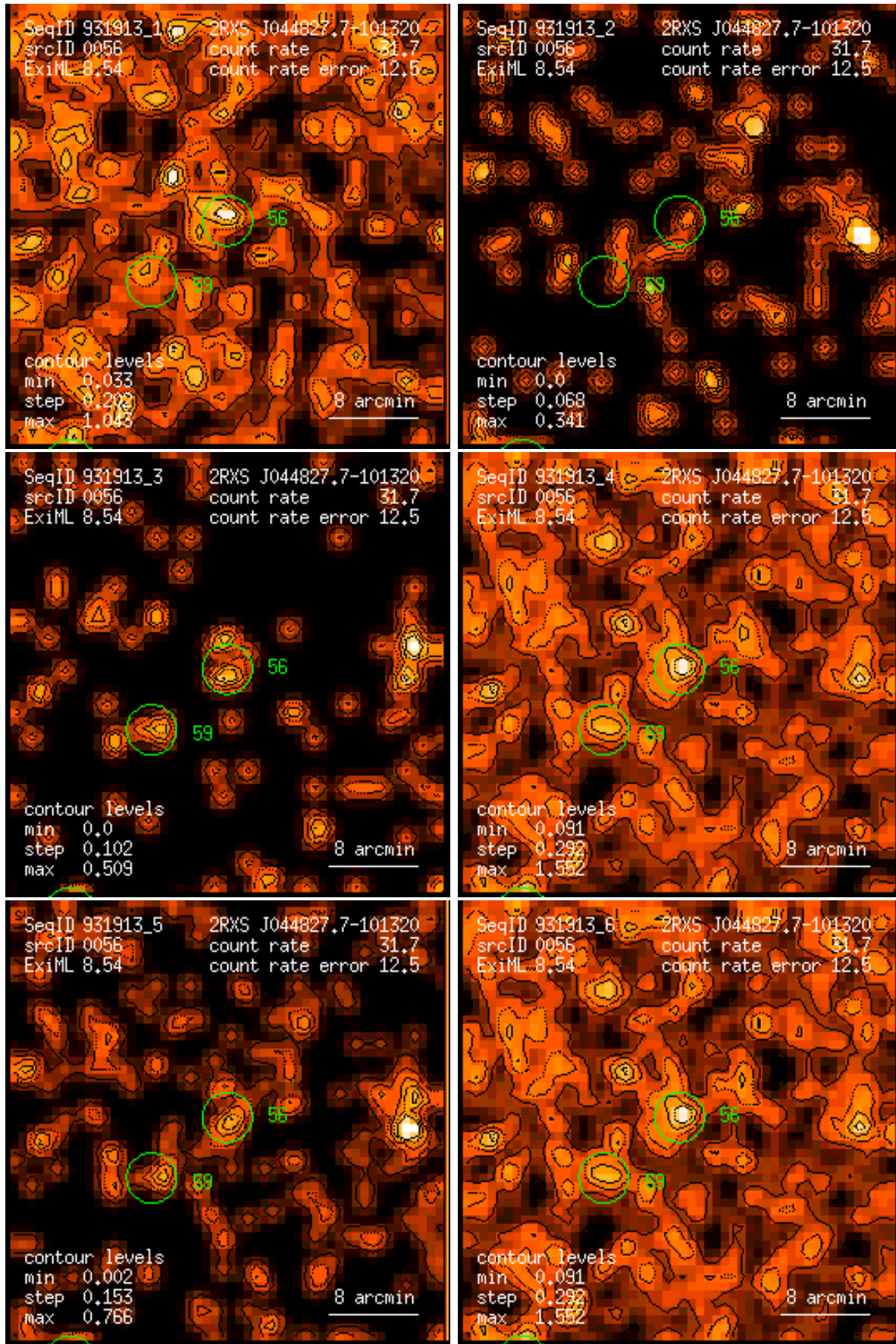
Figure 56: RASS 931913: detection 0056: band rate images, Gaussian filter: (1) PSPC channels 11 – 41, (2) 52 – 90, (3) 91 – 201, (4) 11 – 235, (5) 52 – 201, (6) 11 – 201. Broad band rates in counts/ks. Band rate contour levels in counts/ks/arcmin 2 .
