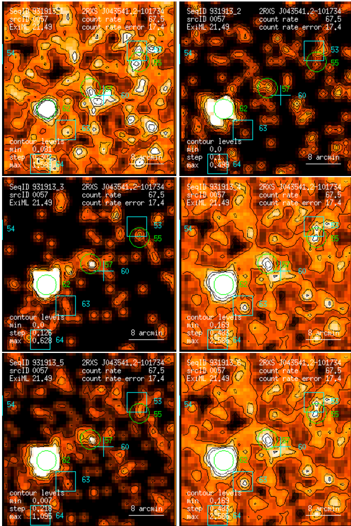
Figure 57: RASS 931913: detection 0057: band rate images, Gaussian filter: (1) PSPC channels 11 – 41, (2) 52 – 90, (3) 91 – 201, (4) 11 – 235, (5) 52 – 201, (6) 11 – 201. Broad band rates in counts/ks. Band rate contour levels in counts/ks/arcmin 2 .
