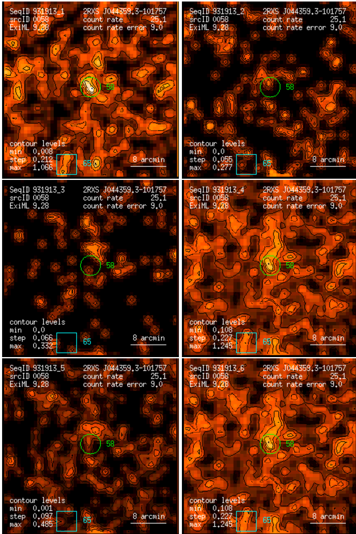
Figure 58: RASS 931913: detection 0058: band rate images, Gaussian filter: (1) PSPC channels 11 – 41, (2) 52 – 90, (3) 91 – 201, (4) 11 – 235, (5) 52 – 201, (6) 11 – 201. Broad band rates in counts/ks. Band rate contour levels in counts/ks/arcmin 2 .
