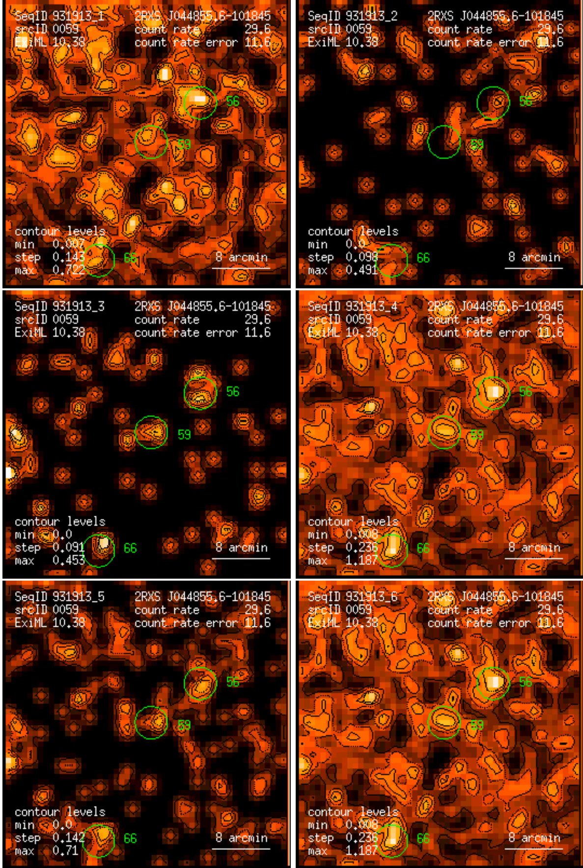
Figure 59: RASS 931913: detection 0059: band rate images, Gaussian filter: (1) PSPC channels 11 – 41, (2) 52 – 90, (3) 91 – 201, (4) 11 – 235, (5) 52 – 201, (6) 11 – 201. Broad band rates in counts/ks. Band rate contour levels in counts/ks/arcmin 2 .
