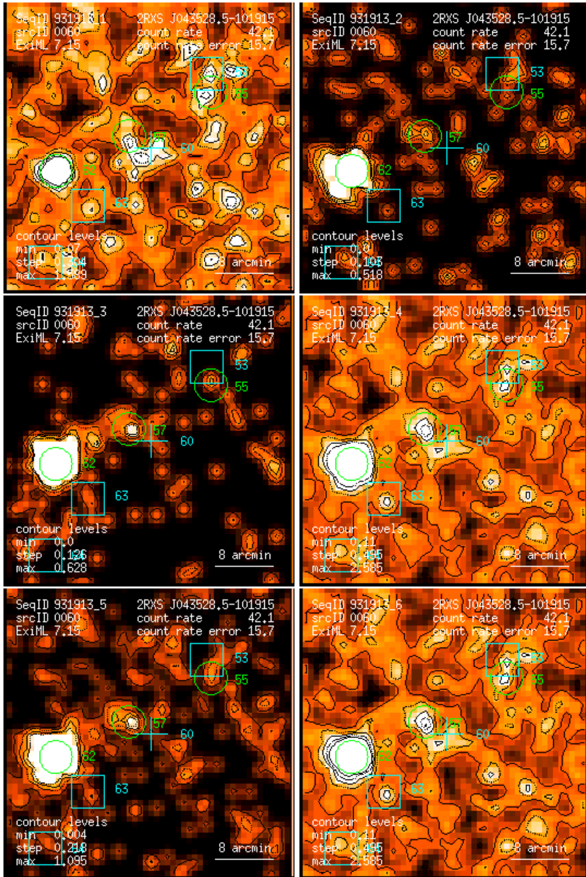
Figure 60: RASS 931913: detection 0060: band rate images, Gaussian filter: (1) PSPC channels 11 – 41, (2) 52 – 90, (3) 91 – 201, (4) 11 – 235, (5) 52 – 201, (6) 11 – 201. Broad band rates in counts/ks. Band rate contour levels in counts/ks/arcmin 2 .
