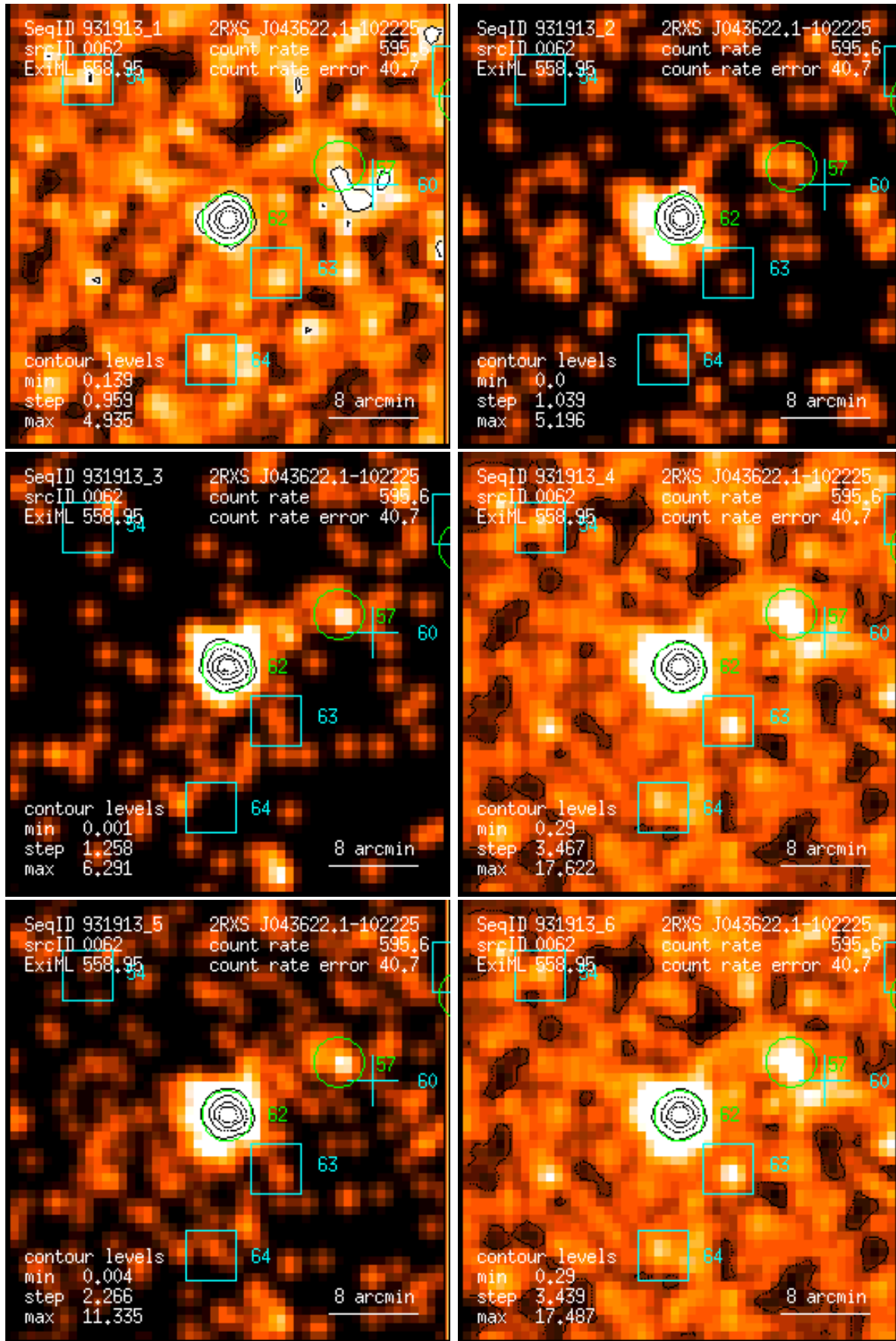
Figure 62: RASS 931913: detection 0062: band rate images, Gaussian filter: (1) PSPC channels 11 – 41, (2) 52 – 90, (3) 91 – 201, (4) 11 – 235, (5) 52 – 201, (6) 11 – 201. Broad band rates in counts/ks. Band rate contour levels in counts/ks/arcmin 2 .
