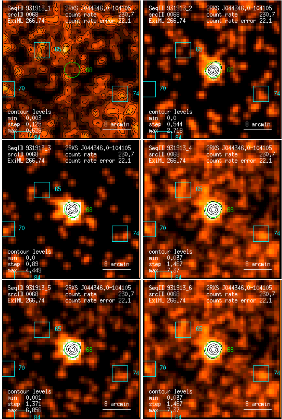
Figure 68: RASS 931913: detection 0068: band rate images, Gaussian filter: (1) PSPC channels 11 – 41, (2) 52 – 90, (3) 91 – 201, (4) 11 – 235, (5) 52 – 201, (6) 11 – 201. Broad band rates in counts/ks. Band rate contour levels in counts/ks/arcmin 2 .
