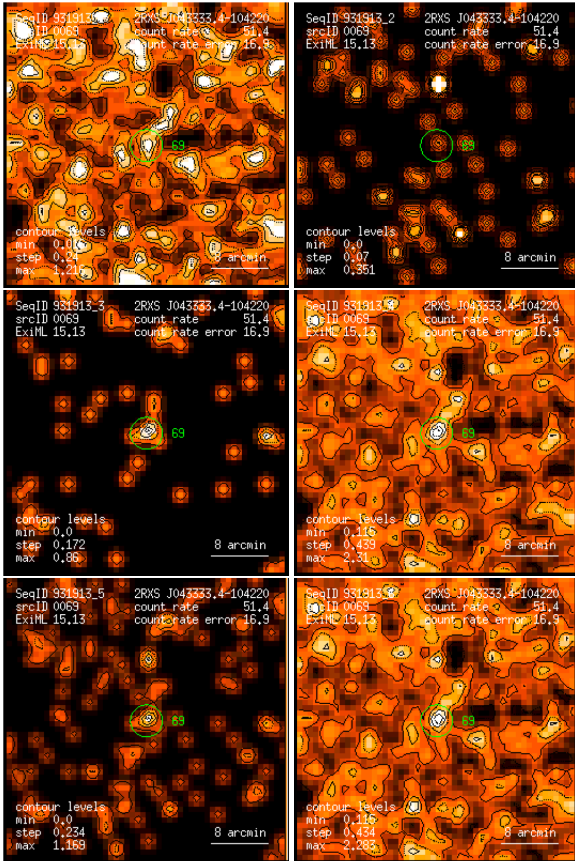
Figure 69: RASS 931913: detection 0069: band rate images, Gaussian filter: (1) PSPC channels 11 – 41, (2) 52 – 90, (3) 91 – 201, (4) 11 – 235, (5) 52 – 201, (6) 11 – 201. Broad band rates in counts/ks. Band rate contour levels in counts/ks/arcmin 2 .
