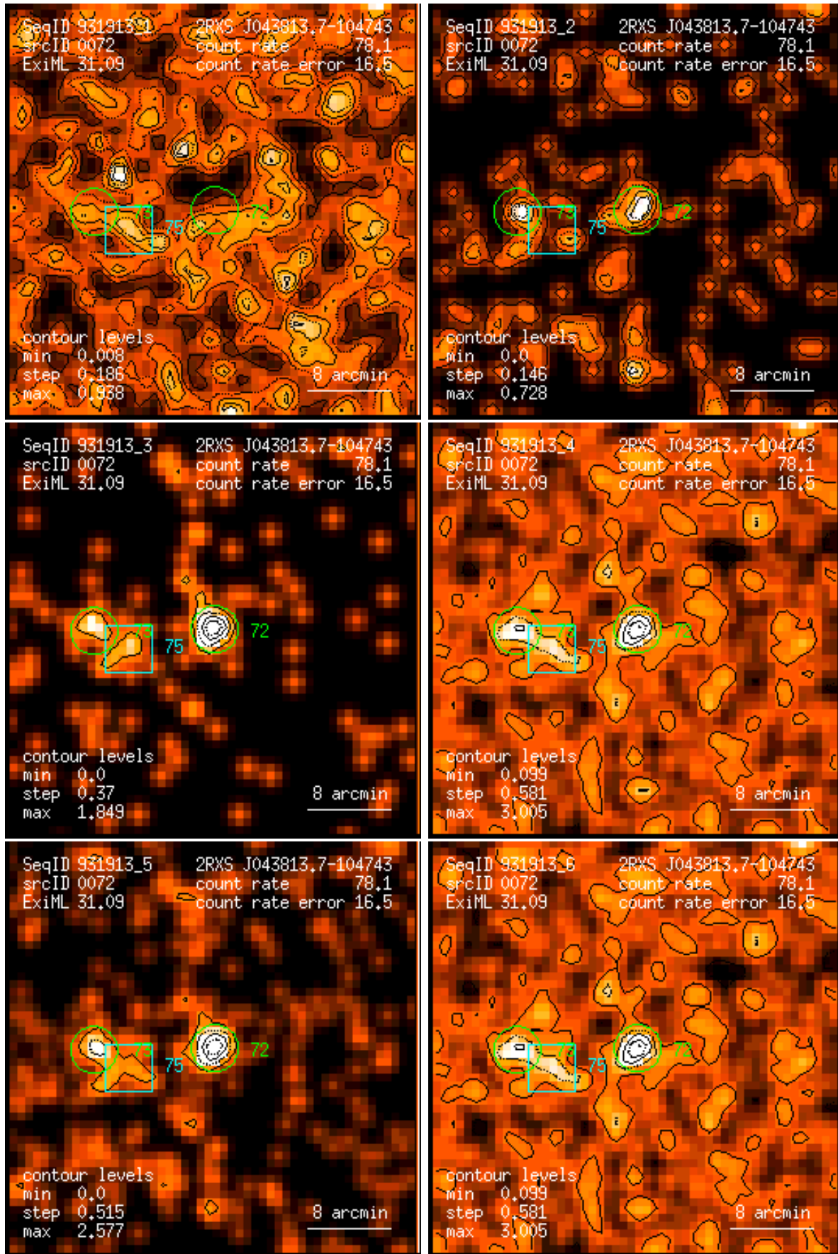
Figure 72: RASS 931913: detection 0072: band rate images, Gaussian filter: (1) PSPC channels 11 – 41, (2) 52 – 90, (3) 91 – 201, (4) 11 – 235, (5) 52 – 201, (6) 11 – 201. Broad band rates in counts/ks. Band rate contour levels in counts/ks/arcmin 2 .
