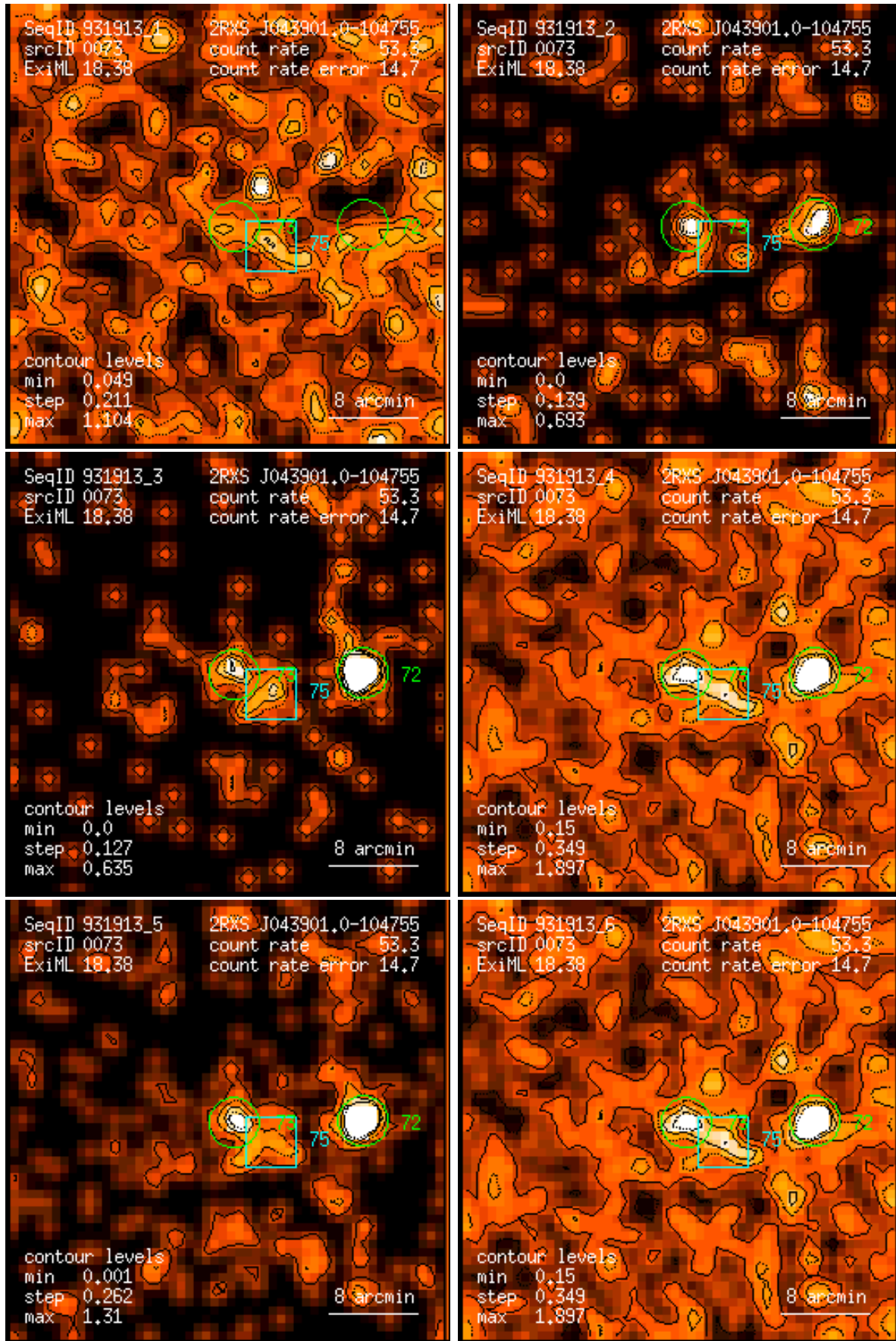
Figure 73: RASS 931913: detection 0073: band rate images, Gaussian filter: (1) PSPC channels 11 – 41, (2) 52 – 90, (3) 91 – 201, (4) 11 – 235, (5) 52 – 201, (6) 11 – 201. Broad band rates in counts/ks. Band rate contour levels in counts/ks/arcmin 2 .
