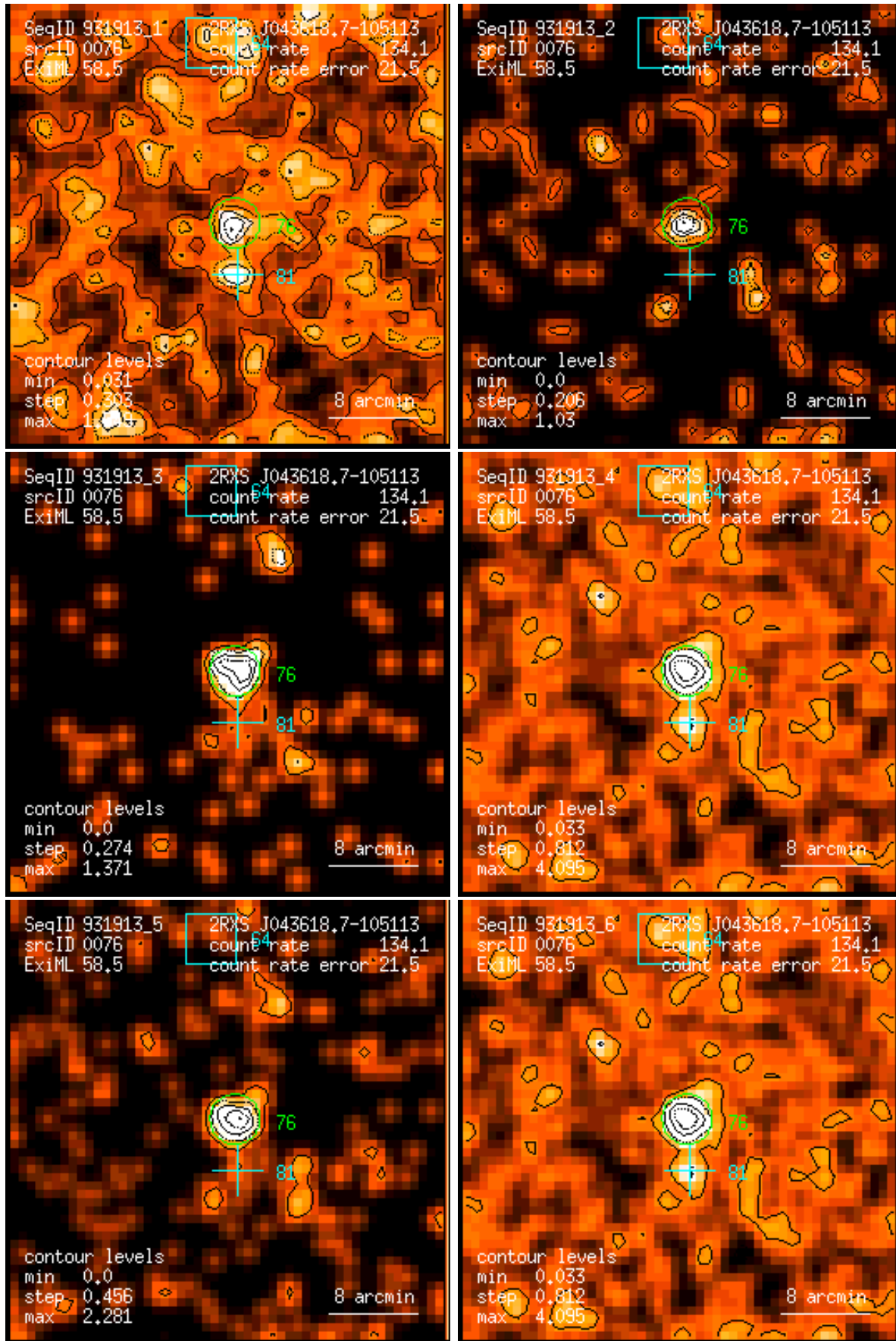
Figure 76: RASS 931913: detection 0076: band rate images, Gaussian filter: (1) PSPC channels 11 – 41, (2) 52 – 90, (3) 91 – 201, (4) 11 – 235, (5) 52 – 201, (6) 11 – 201. Broad band rates in counts/ks. Band rate contour levels in counts/ks/arcmin 2 .
