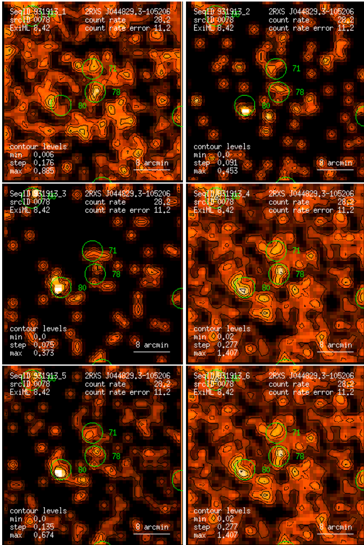
Figure 78: RASS 931913: detection 0078: band rate images, Gaussian filter: (1) PSPC channels 11 – 41, (2) 52 – 90, (3) 91 – 201, (4) 11 – 235, (5) 52 – 201, (6) 11 – 201. Broad band rates in counts/ks. Band rate contour levels in counts/ks/arcmin 2 .
