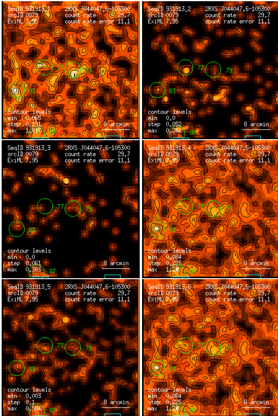
Figure 79: RASS 931913: detection 0079: band rate images, Gaussian filter: (1) PSPC channels 11 – 41, (2) 52 – 90, (3) 91 – 201, (4) 11 – 235, (5) 52 – 201, (6) 11 – 201. Broad band rates in counts/ks. Band rate contour levels in counts/ks/arcmin 2 .
