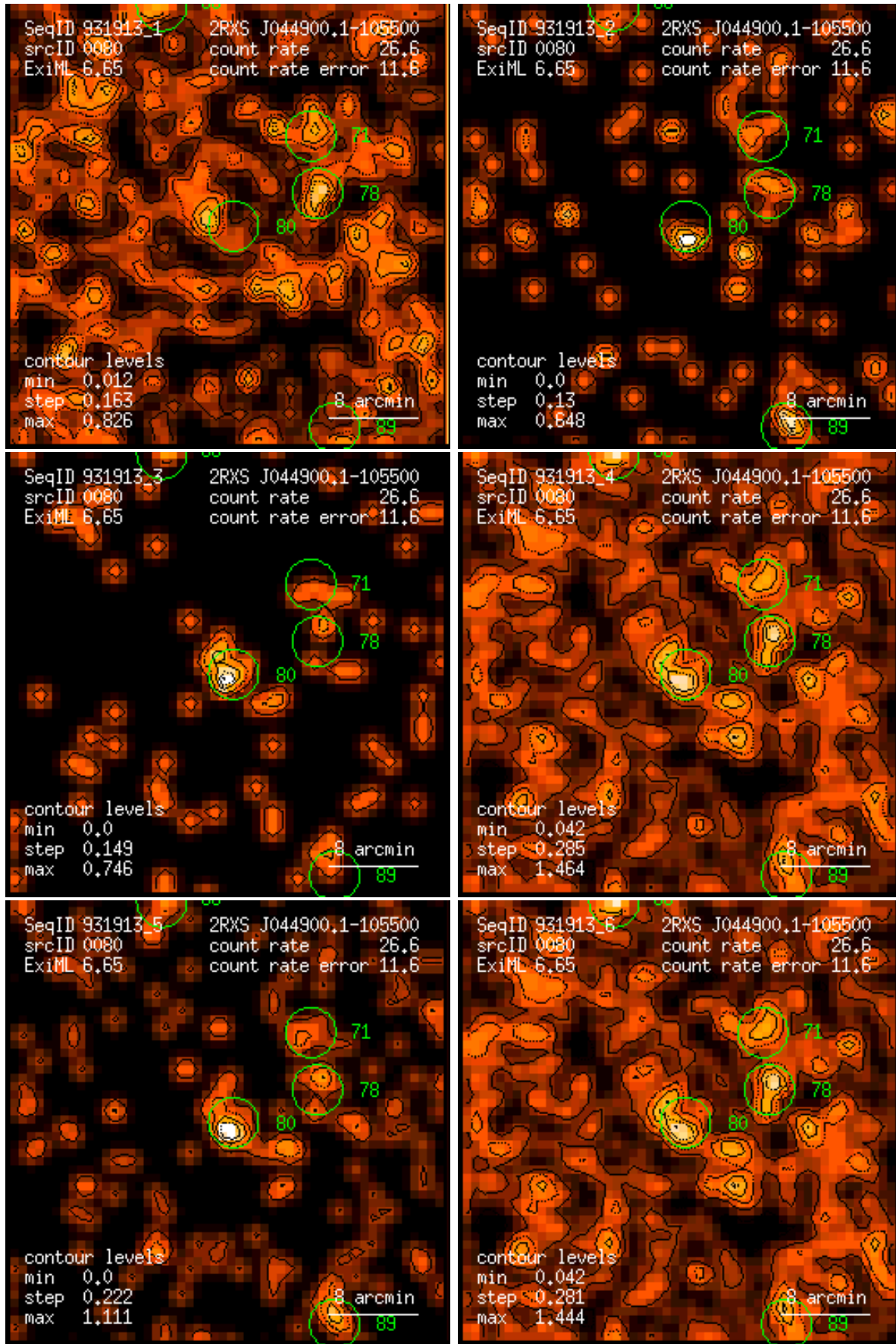
Figure 80: RASS 931913: detection 0080: band rate images, Gaussian filter: (1) PSPC channels 11 – 41, (2) 52 – 90, (3) 91 – 201, (4) 11 – 235, (5) 52 – 201, (6) 11 – 201. Broad band rates in counts/ks. Band rate contour levels in counts/ks/arcmin 2 .
