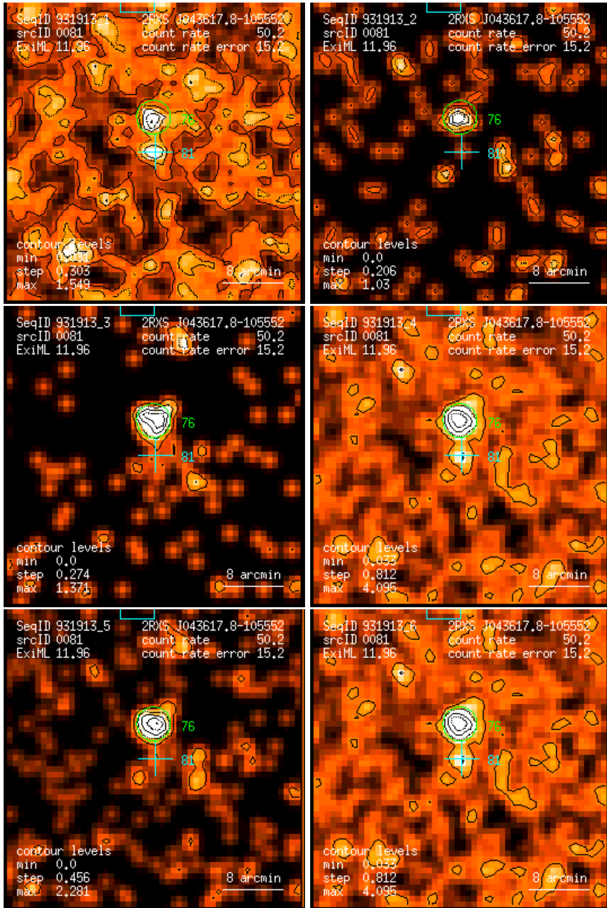
Figure 81: RASS 931913: detection 0081: band rate images, Gaussian filter: (1) PSPC channels 11 – 41, (2) 52 – 90, (3) 91 – 201, (4) 11 – 235, (5) 52 – 201, (6) 11 – 201. Broad band rates in counts/ks. Band rate contour levels in counts/ks/arcmin 2 .
