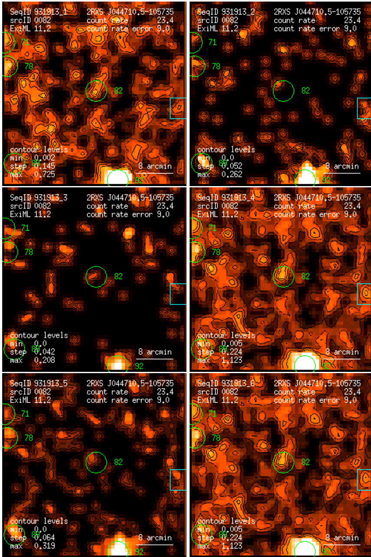
Figure 82: RASS 931913: detection 0082: band rate images, Gaussian filter: (1) PSPC channels 11 – 41, (2) 52 – 90, (3) 91 – 201, (4) 11 – 235, (5) 52 – 201, (6) 11 – 201. Broad band rates in counts/ks. Band rate contour levels in counts/ks/arcmin 2 .
