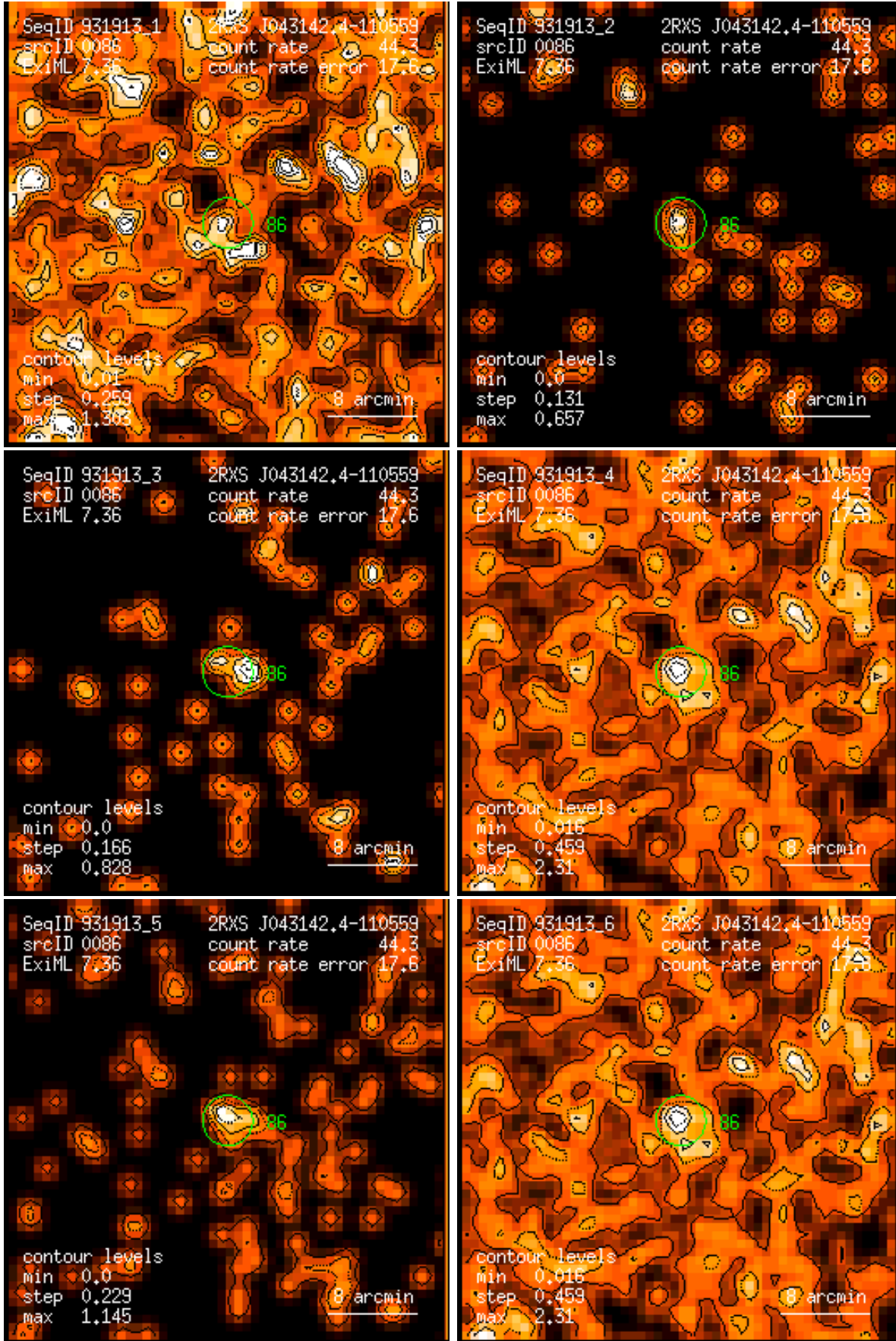
Figure 86: RASS 931913: detection 0086: band rate images, Gaussian filter: (1) PSPC channels 11 – 41, (2) 52 – 90, (3) 91 – 201, (4) 11 – 235, (5) 52 – 201, (6) 11 – 201. Broad band rates in counts/ks. Band rate contour levels in counts/ks/arcmin 2 .
