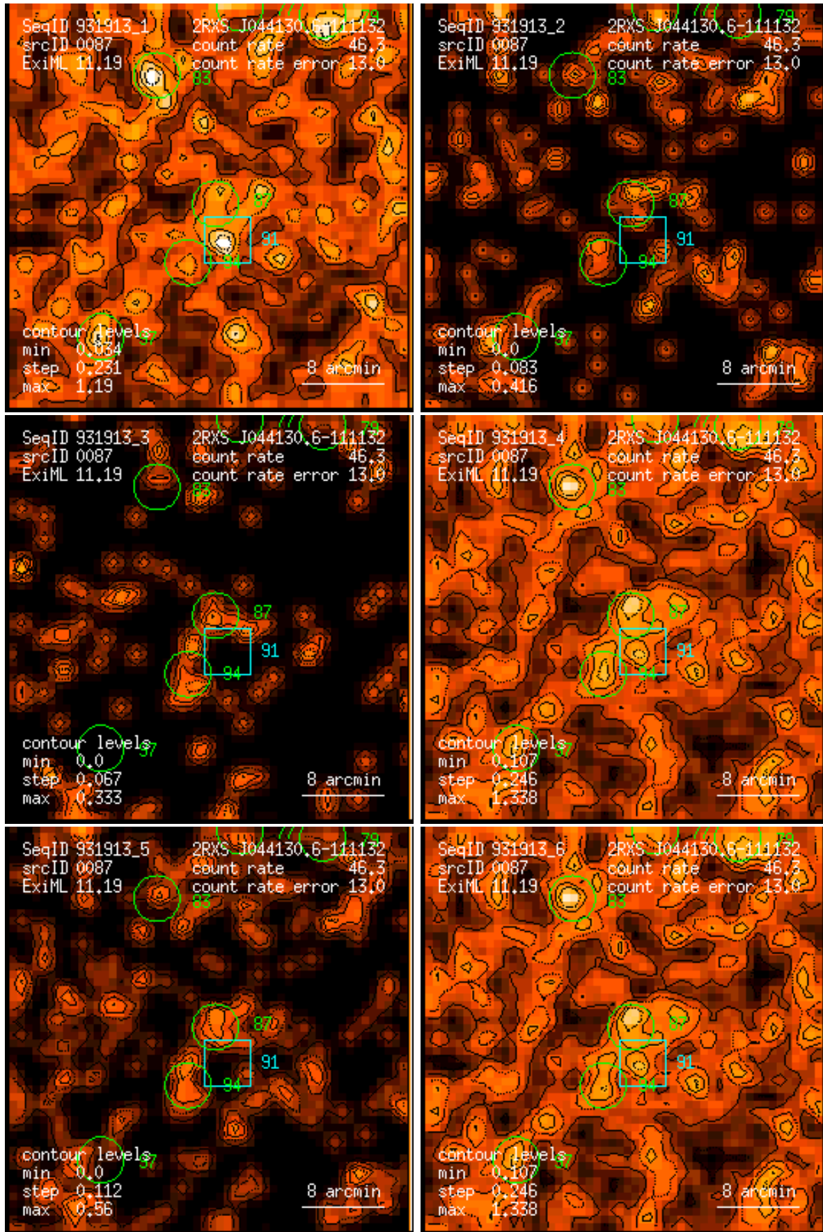
Figure 87: RASS 931913: detection 0087: band rate images, Gaussian filter: (1) PSPC channels 11 – 41, (2) 52 – 90, (3) 91 – 201, (4) 11 – 235, (5) 52 – 201, (6) 11 – 201. Broad band rates in counts/ks. Band rate contour levels in counts/ks/arcmin 2 .
