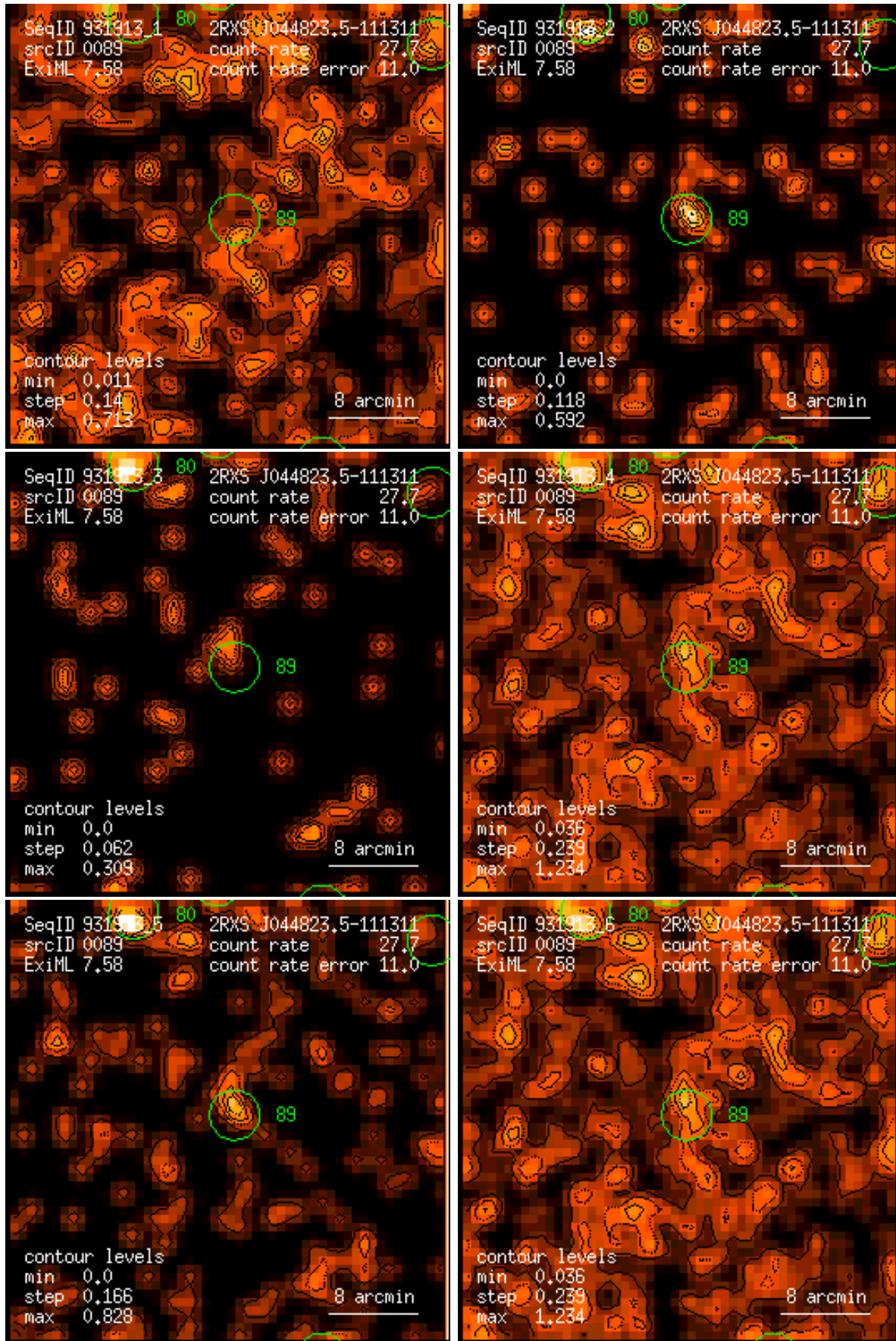
Figure 89: RASS 931913: detection 0089: band rate images, Gaussian filter: (1) PSPC channels 11 – 41, (2) 52 – 90, (3) 91 – 201, (4) 11 – 235, (5) 52 – 201, (6) 11 – 201. Broad band rates in counts/ks. Band rate contour levels in counts/ks/arcmin 2 .
