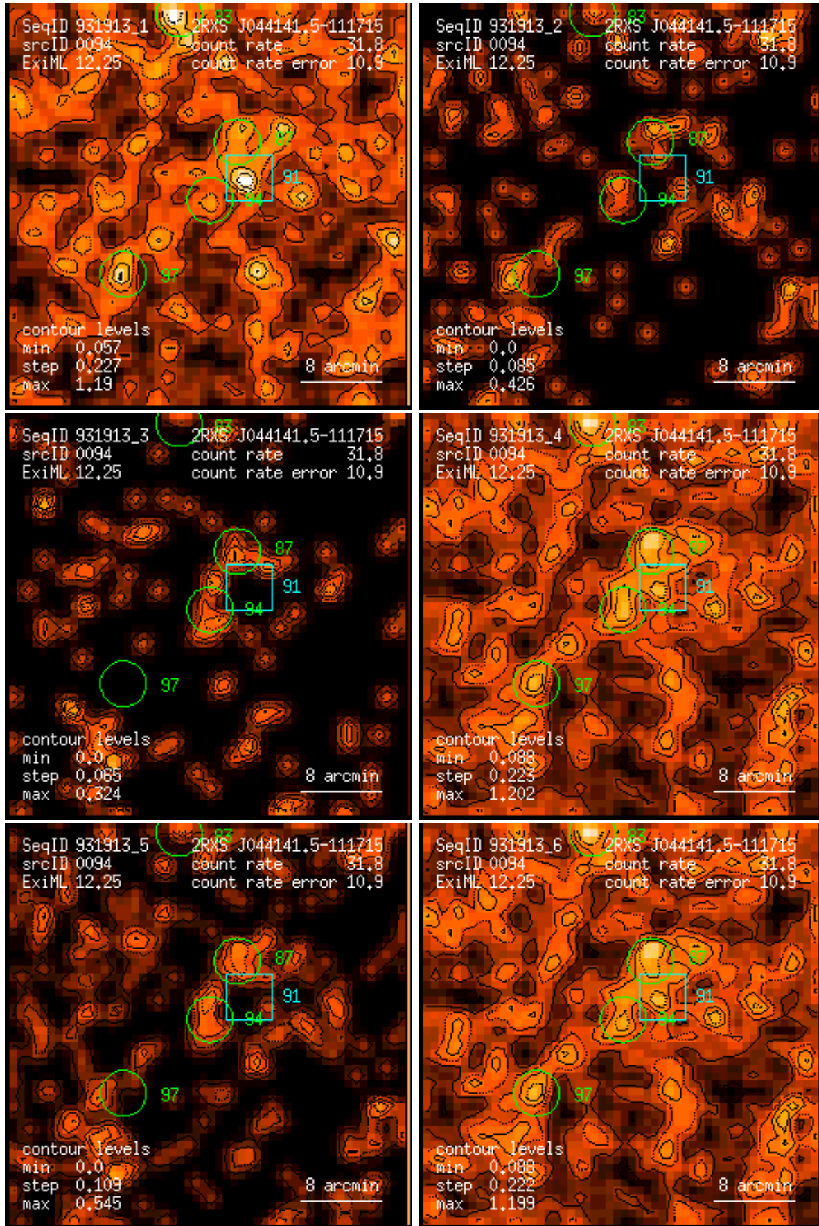
Figure 94: RASS 931913: detection 0094: band rate images, Gaussian filter: (1) PSPC channels 11 – 41, (2) 52 – 90, (3) 91 – 201, (4) 11 – 235, (5) 52 – 201, (6) 11 – 201. Broad band rates in counts/ks. Band rate contour levels in counts/ks/arcmin 2 .
