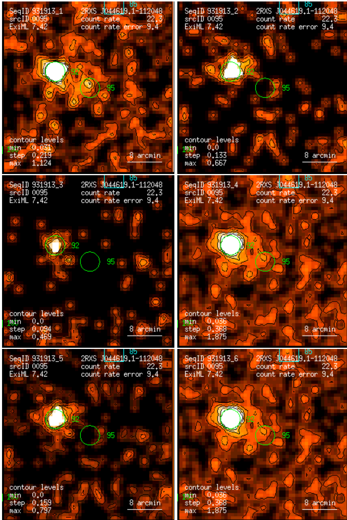
Figure 95: RASS 931913: detection 0095: band rate images, Gaussian filter: (1) PSPC channels 11 – 41, (2) 52 – 90, (3) 91 – 201, (4) 11 – 235, (5) 52 – 201, (6) 11 – 201. Broad band rates in counts/ks. Band rate contour levels in counts/ks/arcmin 2 .
