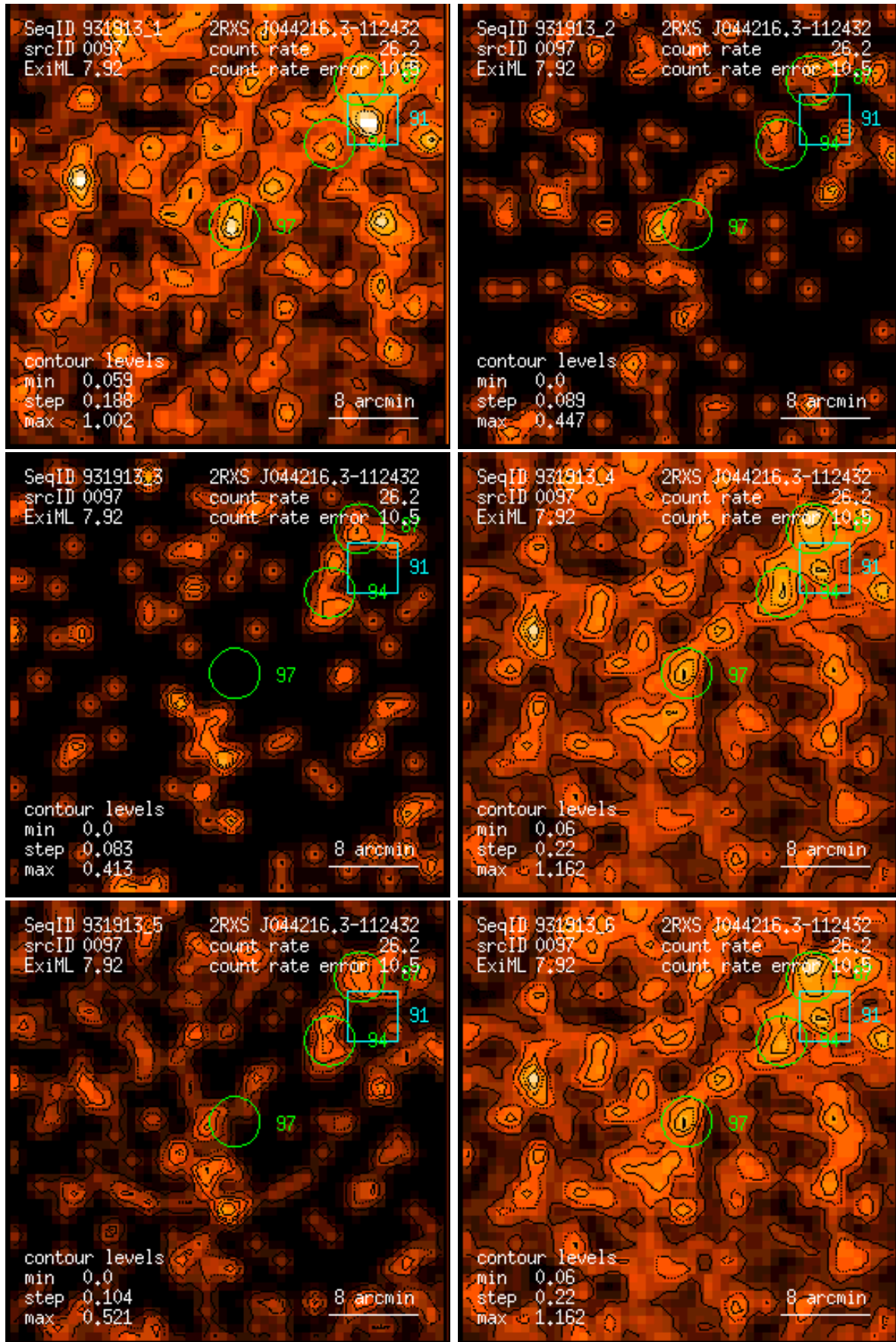
Figure 97: RASS 931913: detection 0097: band rate images, Gaussian filter: (1) PSPC channels 11 – 41, (2) 52 – 90, (3) 91 – 201, (4) 11 – 235, (5) 52 – 201, (6) 11 – 201. Broad band rates in counts/ks. Band rate contour levels in counts/ks/arcmin 2 .
