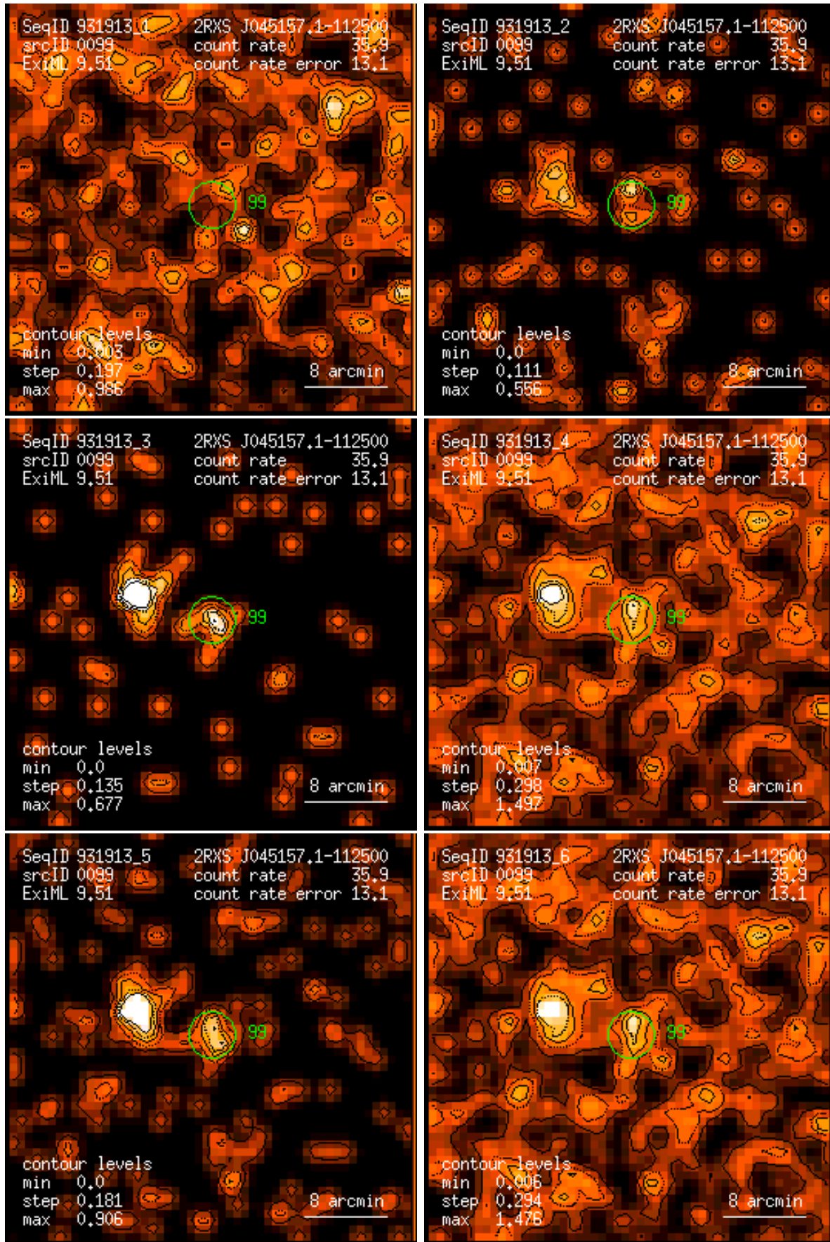
Figure 99: RASS 931913: detection 0099: band rate images, Gaussian filter: (1) PSPC channels 11 – 41, (2) 52 – 90, (3) 91 – 201, (4) 11 – 235, (5) 52 – 201, (6) 11 – 201. Broad band rates in counts/ks. Band rate contour levels in counts/ks/arcmin 2 .
