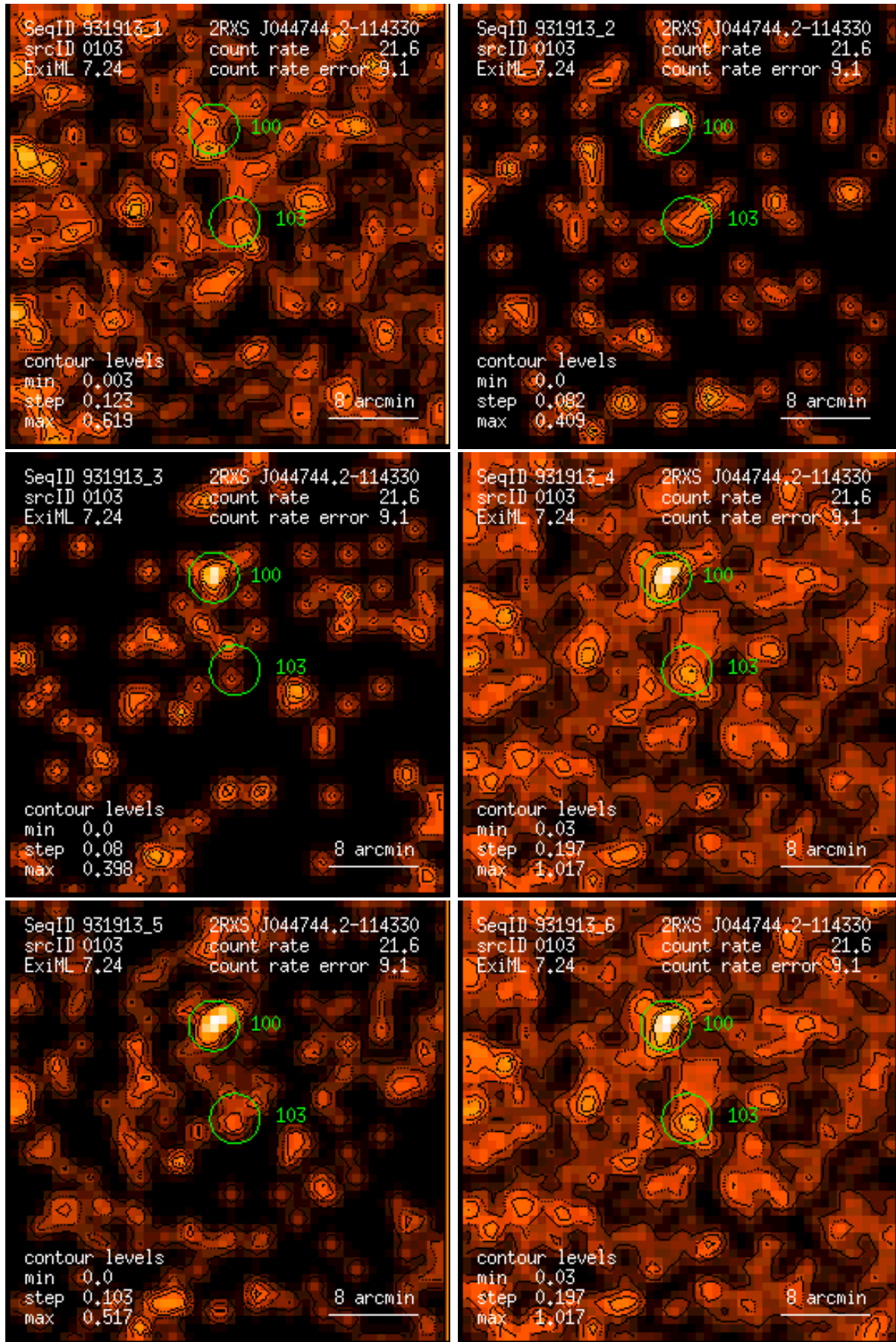
Figure 103: RASS 931913: detection 0103: band rate images, Gaussian filter: (1) PSPC channels 11 – 41, (2) 52 – 90, (3) 91 – 201, (4) 11 – 235, (5) 52 – 201, (6) 11 – 201. Broad band rates in counts/ks. Band rate contour levels in counts/ks/arcmin 2 .
