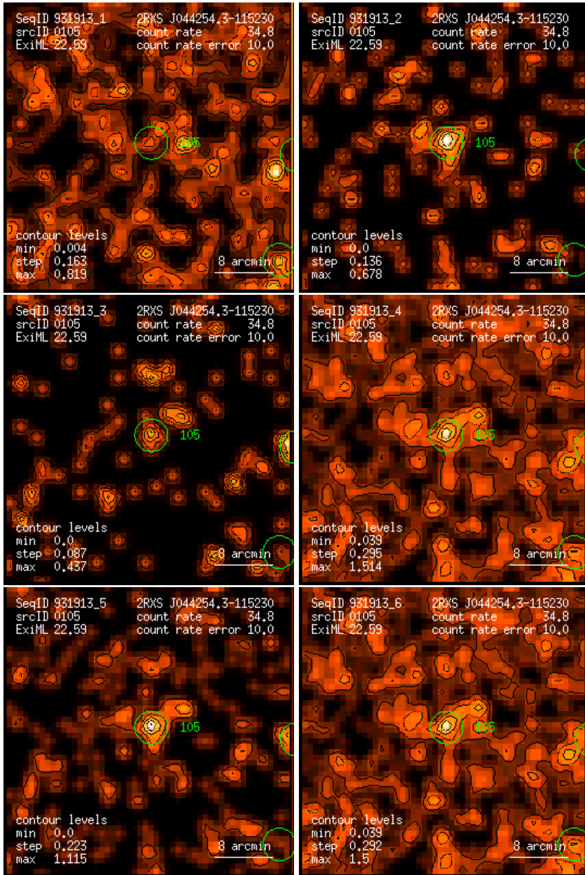
Figure 105: RASS 931913: detection 0105: band rate images, Gaussian filter: (1) PSPC channels 11 – 41, (2) 52 – 90, (3) 91 – 201, (4) 11 – 235, (5) 52 – 201, (6) 11 – 201. Broad band rates in counts/ks. Band rate contour levels in counts/ks/arcmin 2 .
