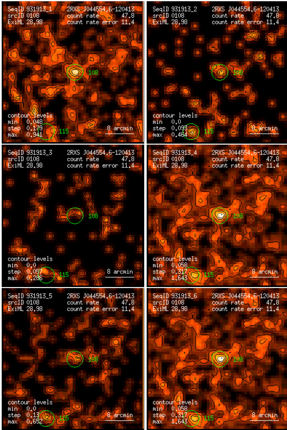
Figure 108: RASS 931913: detection 0108: band rate images, Gaussian filter: (1) PSPC channels 11 – 41, (2) 52 – 90, (3) 91 – 201, (4) 11 – 235, (5) 52 – 201, (6) 11 – 201. Broad band rates in counts/ks. Band rate contour levels in counts/ks/arcmin 2 .
