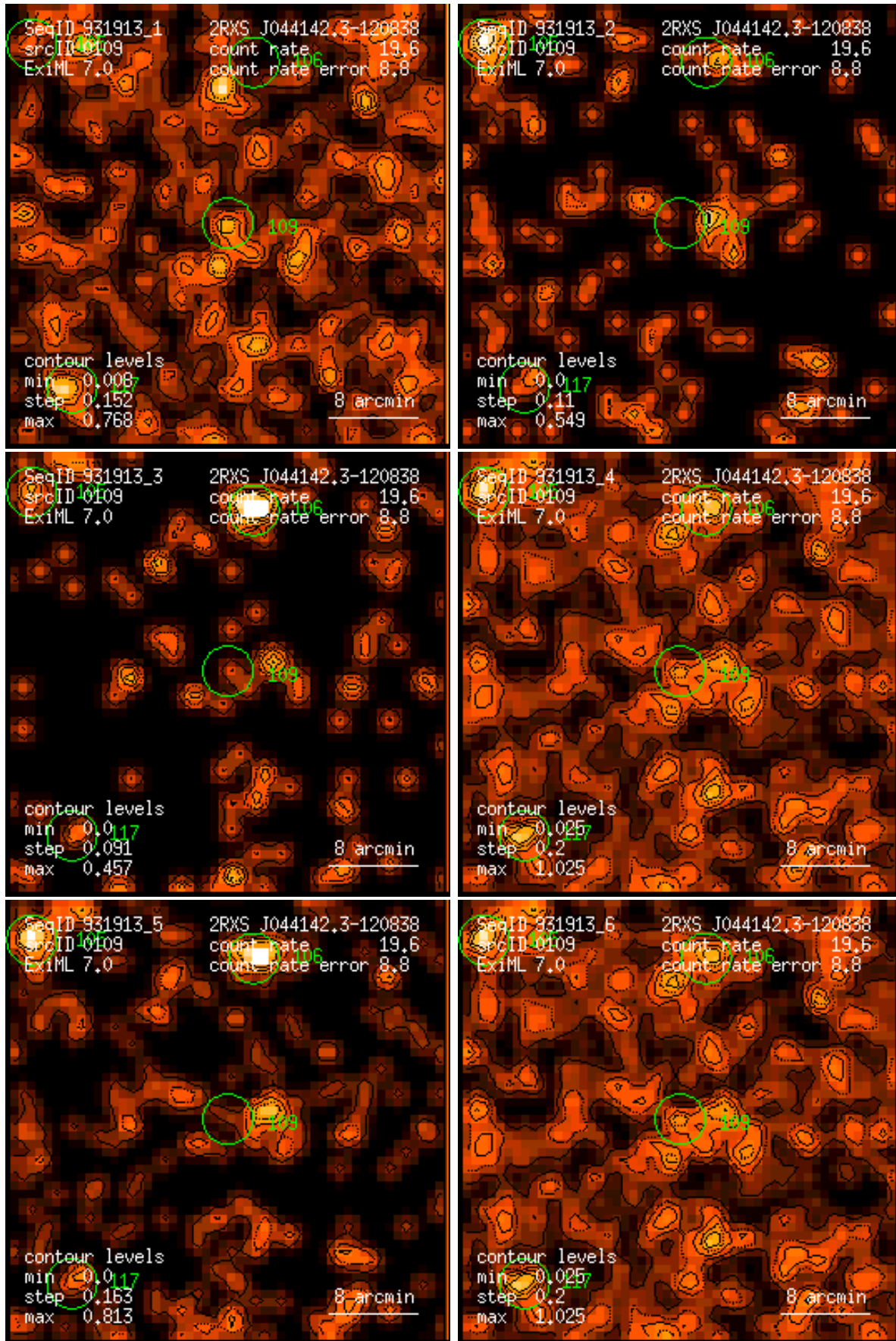
Figure 109: RASS 931913: detection 0109: band rate images, Gaussian filter: (1) PSPC channels 11 – 41, (2) 52 – 90, (3) 91 – 201, (4) 11 – 235, (5) 52 – 201, (6) 11 – 201. Broad band rates in counts/ks. Band rate contour levels in counts/ks/arcmin 2 .
