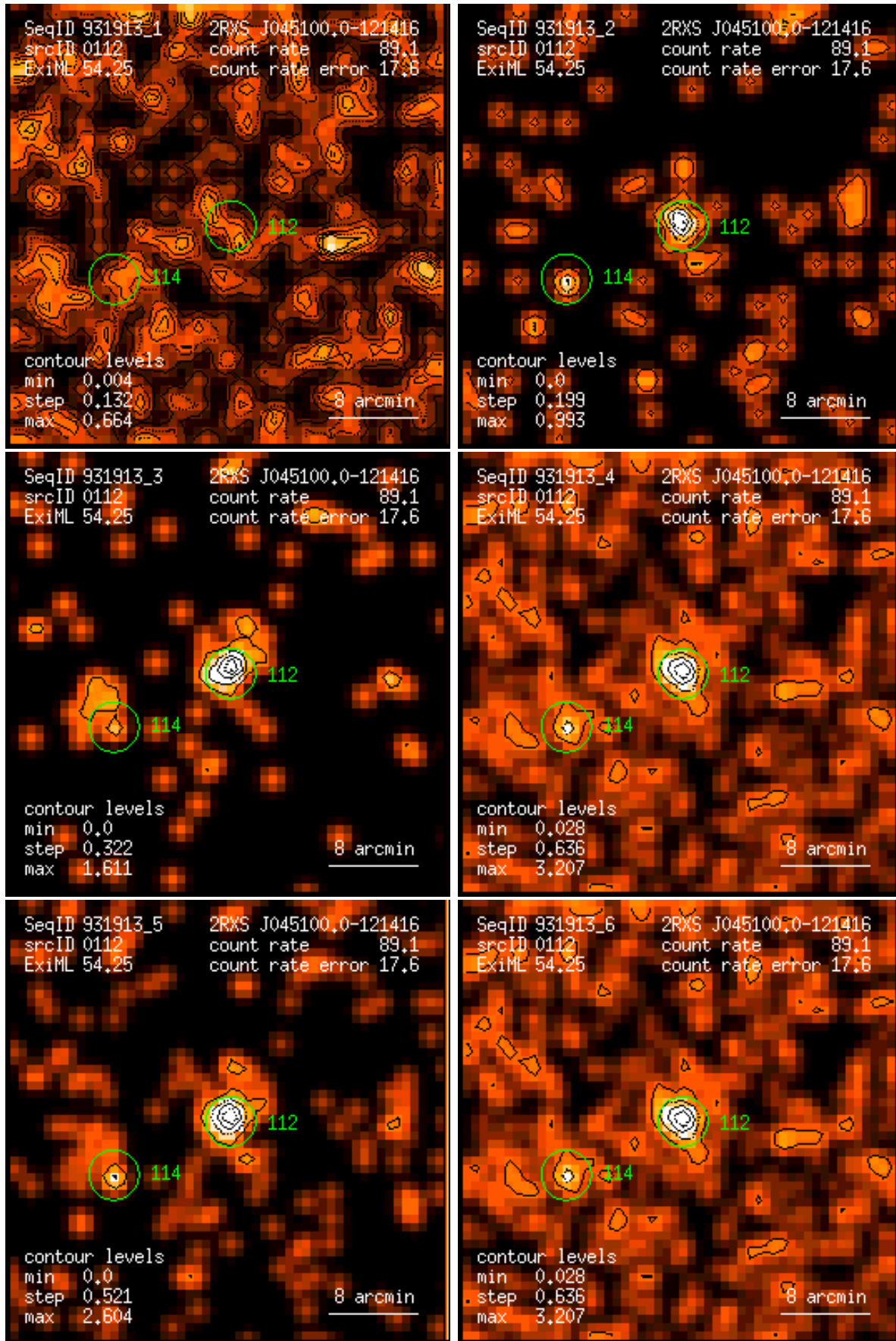
Figure 112: RASS 931913: detection 0112: band rate images, Gaussian filter: (1) PSPC channels 11 – 41, (2) 52 – 90, (3) 91 – 201, (4) 11 – 235, (5) 52 – 201, (6) 11 – 201. Broad band rates in counts/ks. Band rate contour levels in counts/ks/arcmin 2 .
