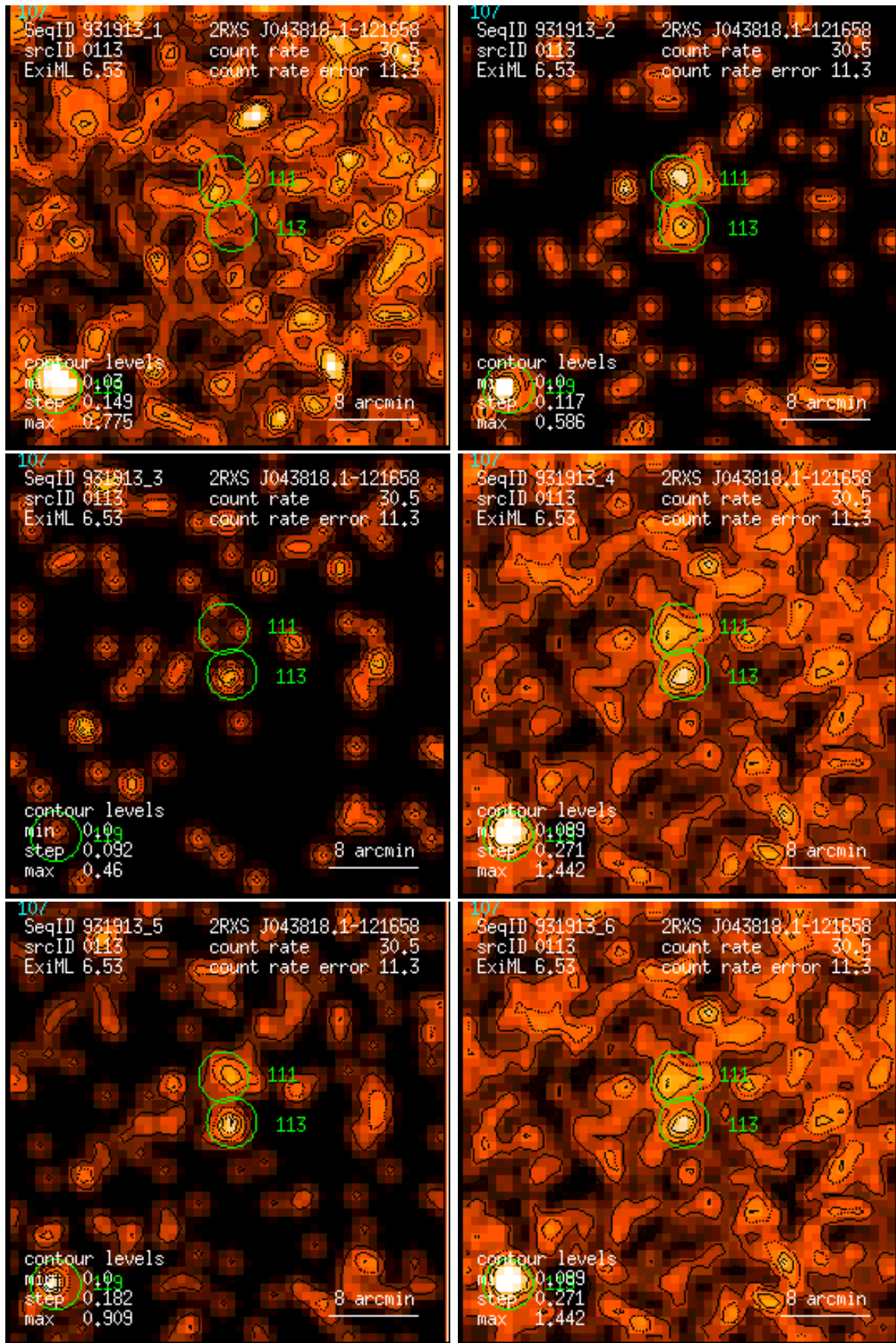
Figure 113: RASS 931913: detection 0113: band rate images, Gaussian filter: (1) PSPC channels 11 – 41, (2) 52 – 90, (3) 91 – 201, (4) 11 – 235, (5) 52 – 201, (6) 11 – 201. Broad band rates in counts/ks. Band rate contour levels in counts/ks/arcmin 2 .
