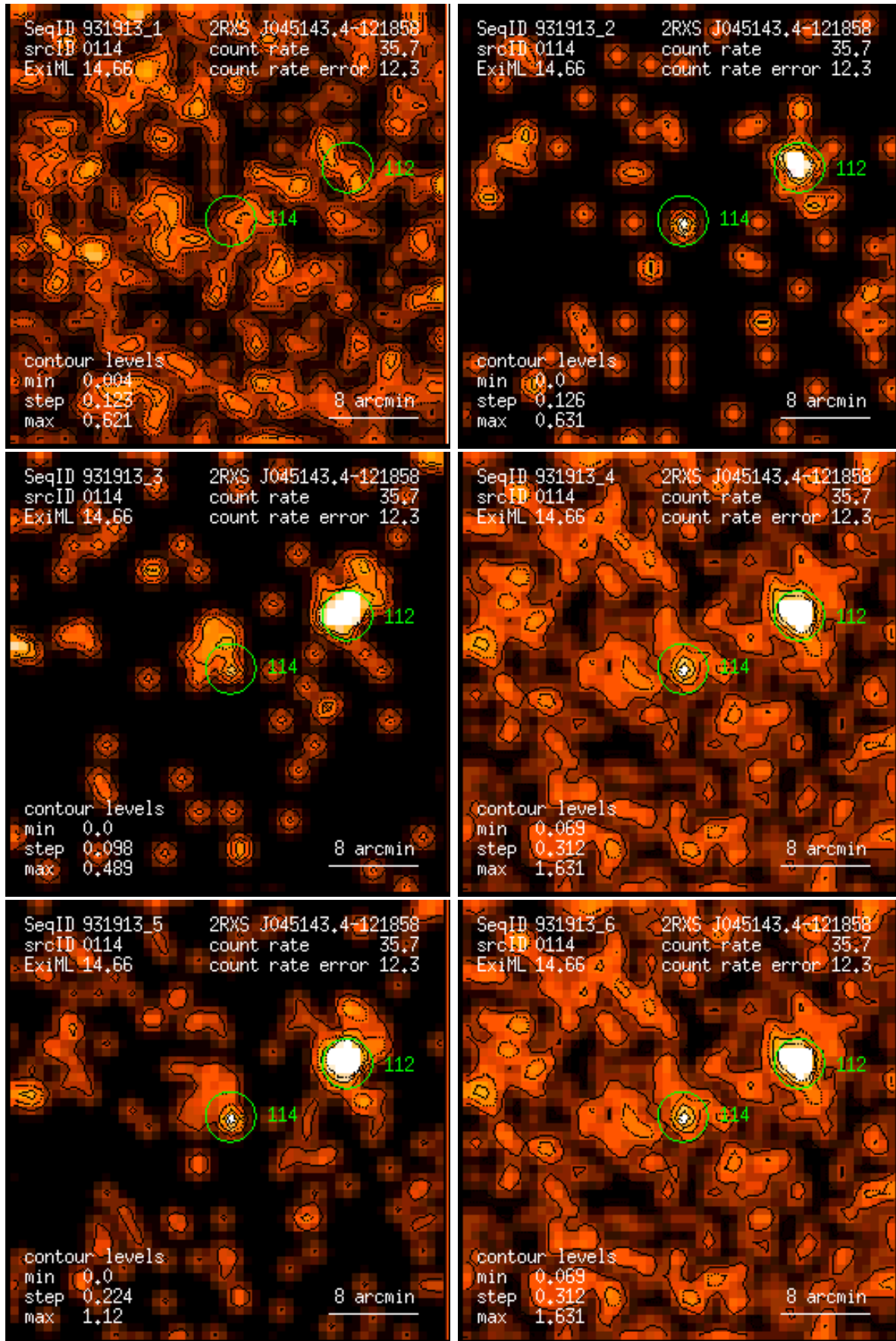
Figure 114: RASS 931913: detection 0114: band rate images, Gaussian filter: (1) PSPC channels 11 – 41, (2) 52 – 90, (3) 91 – 201, (4) 11 – 235, (5) 52 – 201, (6) 11 – 201. Broad band rates in counts/ks. Band rate contour levels in counts/ks/arcmin 2 .
