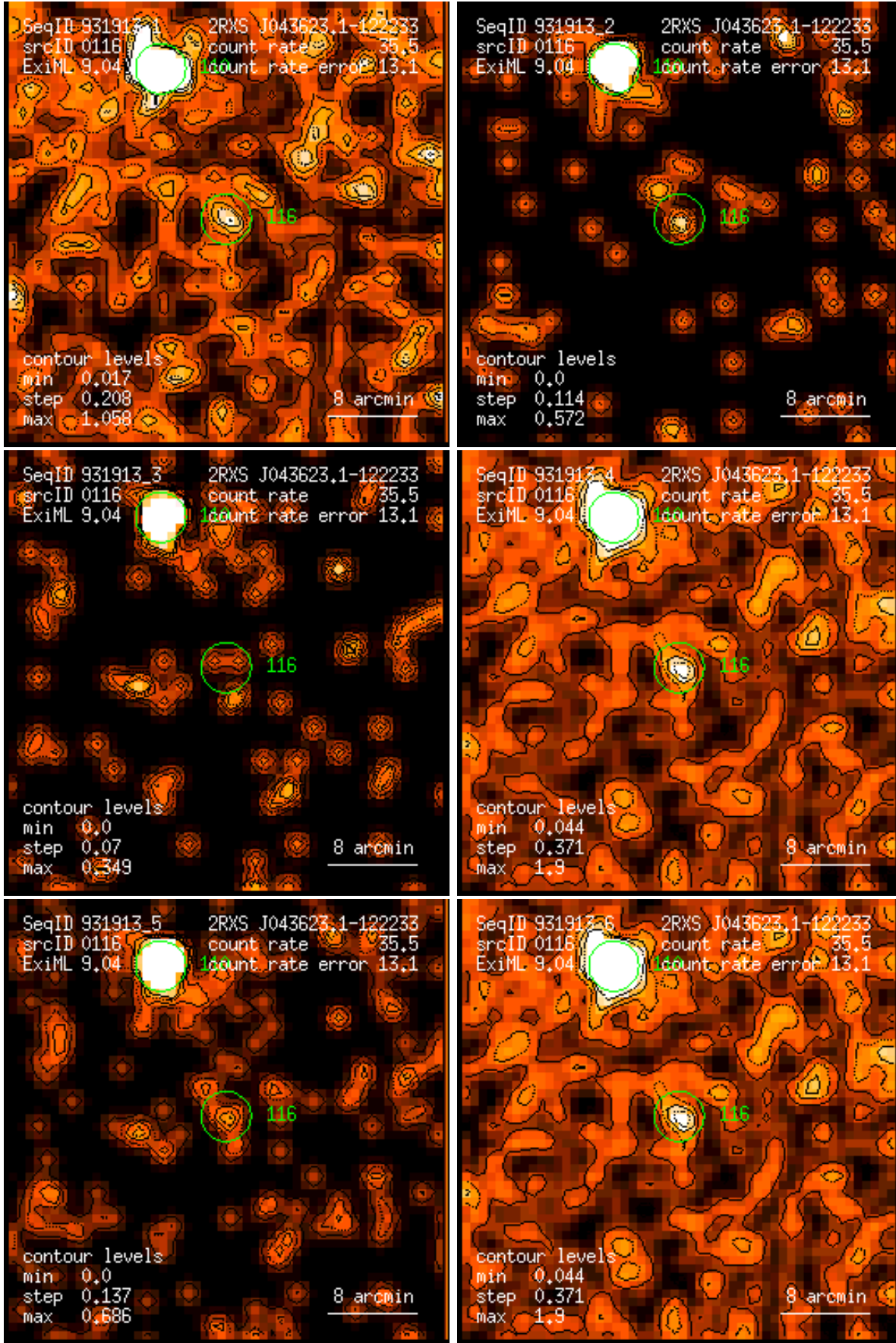
Figure 116: RASS 931913: detection 0116: band rate images, Gaussian filter: (1) PSPC channels 11 – 41, (2) 52 – 90, (3) 91 – 201, (4) 11 – 235, (5) 52 – 201, (6) 11 – 201. Broad band rates in counts/ks. Band rate contour levels in counts/ks/arcmin 2 .
