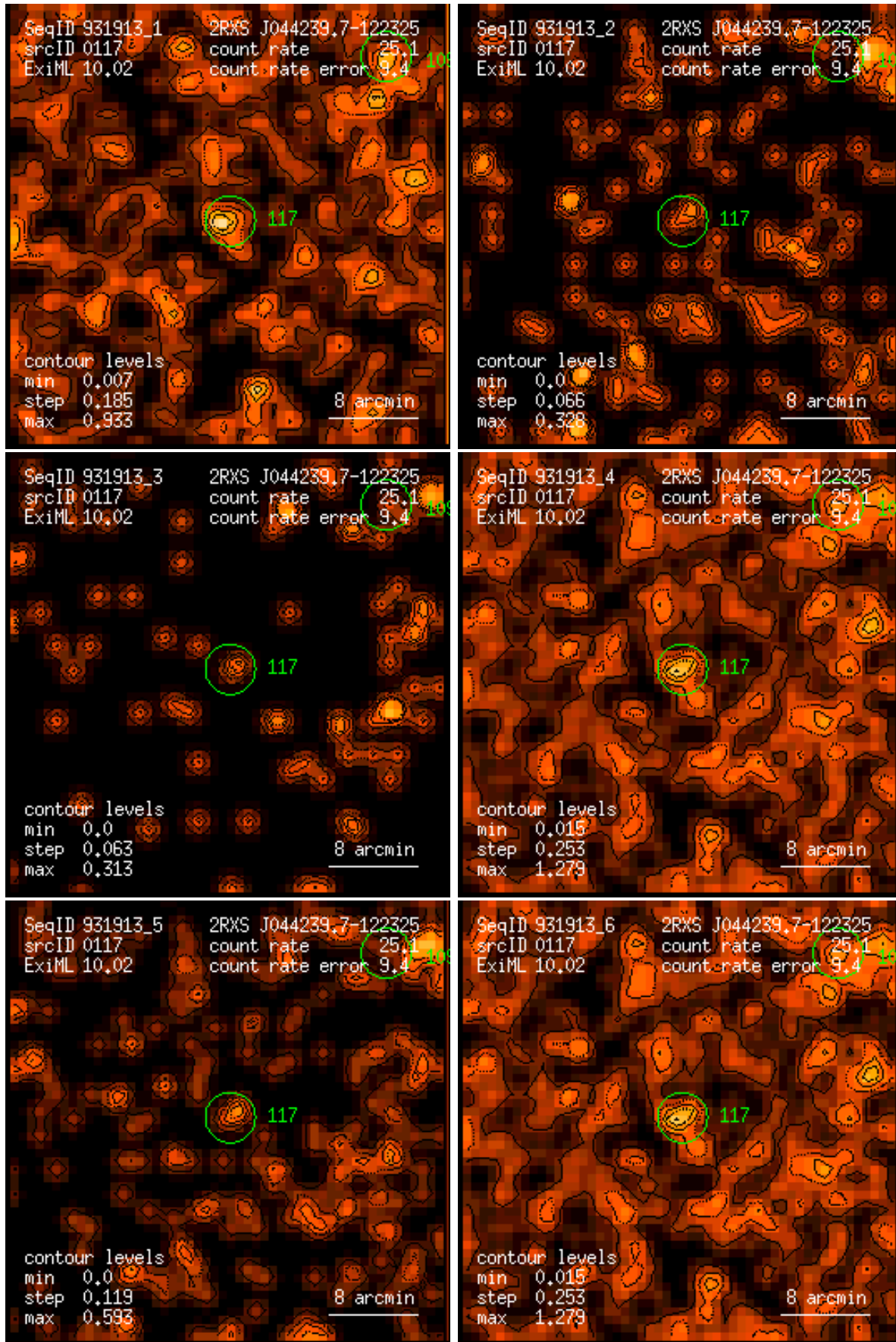
Figure 117: RASS 931913: detection 0117: band rate images, Gaussian filter: (1) PSPC channels 11 – 41, (2) 52 – 90, (3) 91 – 201, (4) 11 – 235, (5) 52 – 201, (6) 11 – 201. Broad band rates in counts/ks. Band rate contour levels in counts/ks/arcmin 2 .
