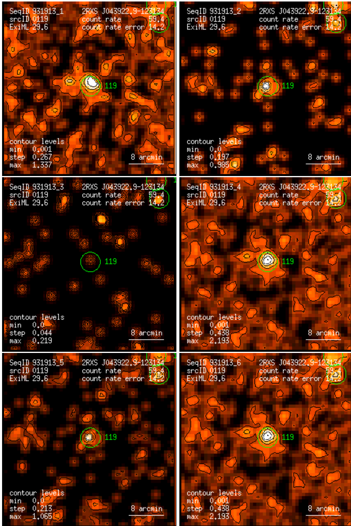
Figure 119: RASS 931913: detection 0119: band rate images, Gaussian filter: (1) PSPC channels 11 – 41, (2) 52 – 90, (3) 91 – 201, (4) 11 – 235, (5) 52 – 201, (6) 11 – 201. Broad band rates in counts/ks. Band rate contour levels in counts/ks/arcmin 2 .
