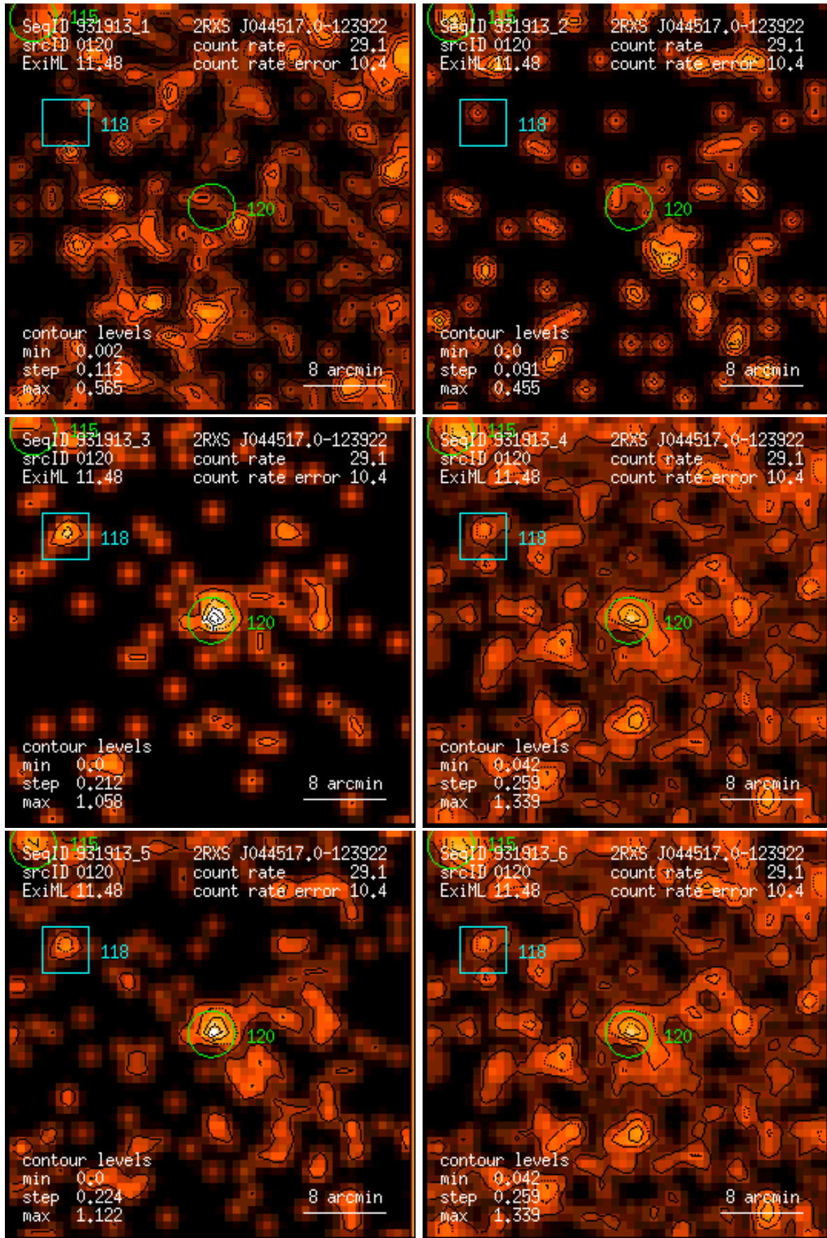
Figure 120: RASS 931913: detection 0120: band rate images, Gaussian filter: (1) PSPC channels 11 – 41, (2) 52 – 90, (3) 91 – 201, (4) 11 – 235, (5) 52 – 201, (6) 11 – 201. Broad band rates in counts/ks. Band rate contour levels in counts/ks/arcmin 2 .
