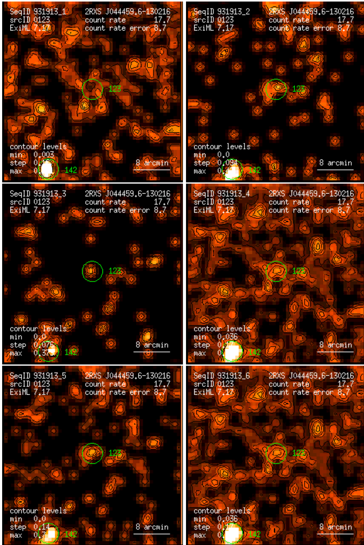
Figure 123: RASS 931913: detection 0123: band rate images, Gaussian filter: (1) PSPC channels 11 – 41, (2) 52 – 90, (3) 91 – 201, (4) 11 – 235, (5) 52 – 201, (6) 11 – 201. Broad band rates in counts/ks. Band rate contour levels in counts/ks/arcmin 2 .
