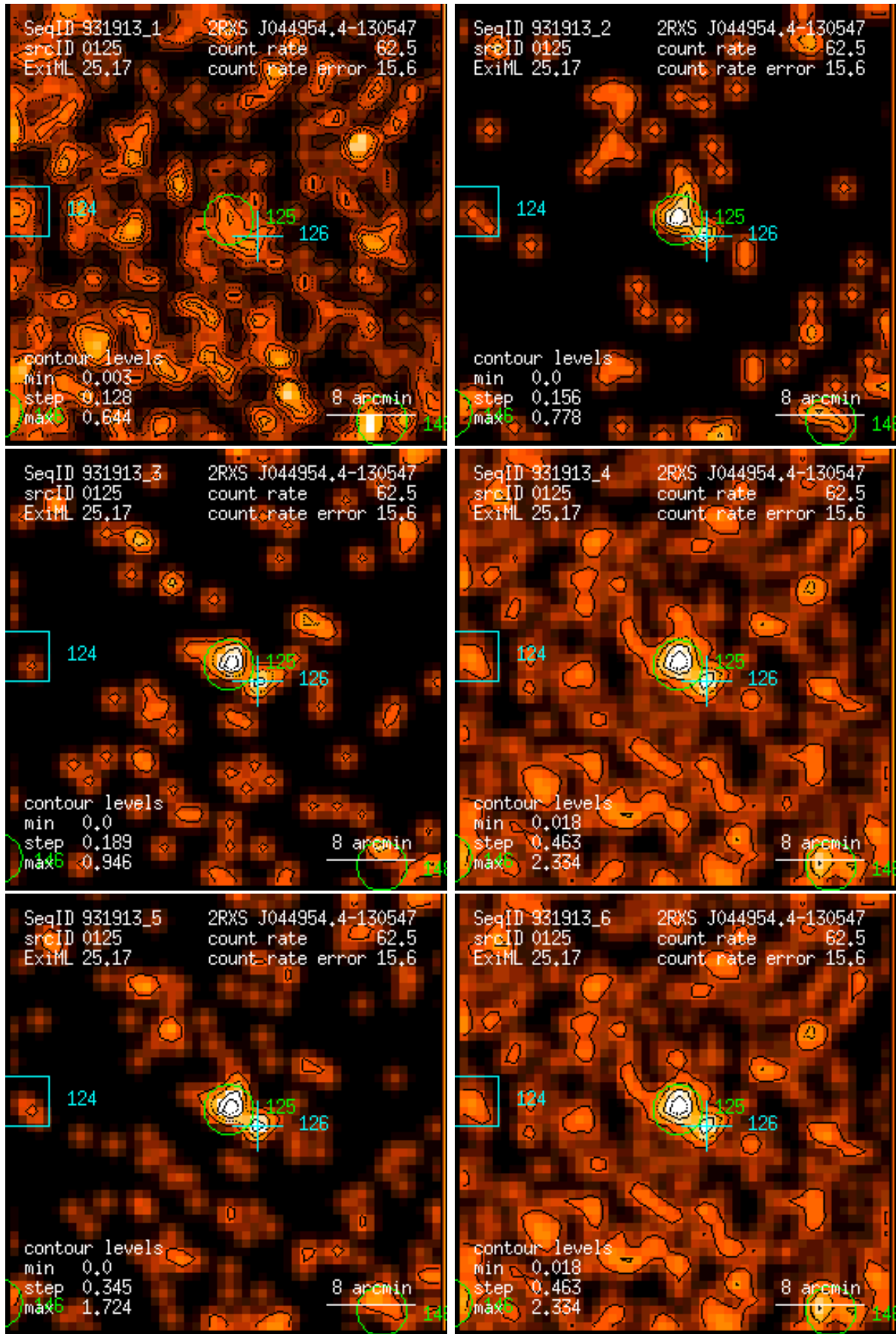
Figure 125: RASS 931913: detection 0125: band rate images, Gaussian filter: (1) PSPC channels 11 – 41, (2) 52 – 90, (3) 91 – 201, (4) 11 – 235, (5) 52 – 201, (6) 11 – 201. Broad band rates in counts/ks. Band rate contour levels in counts/ks/arcmin 2 .
