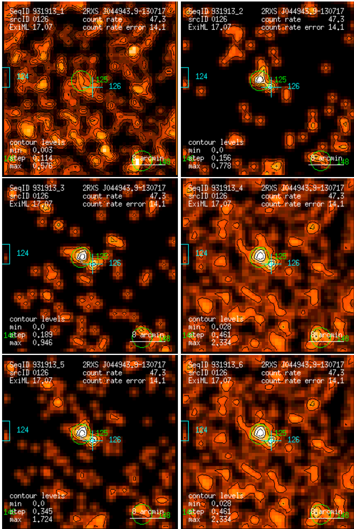
Figure 126: RASS 931913: detection 0126: band rate images, Gaussian filter: (1) PSPC channels 11 – 41, (2) 52 – 90, (3) 91 – 201, (4) 11 – 235, (5) 52 – 201, (6) 11 – 201. Broad band rates in counts/ks. Band rate contour levels in counts/ks/arcmin 2 .
