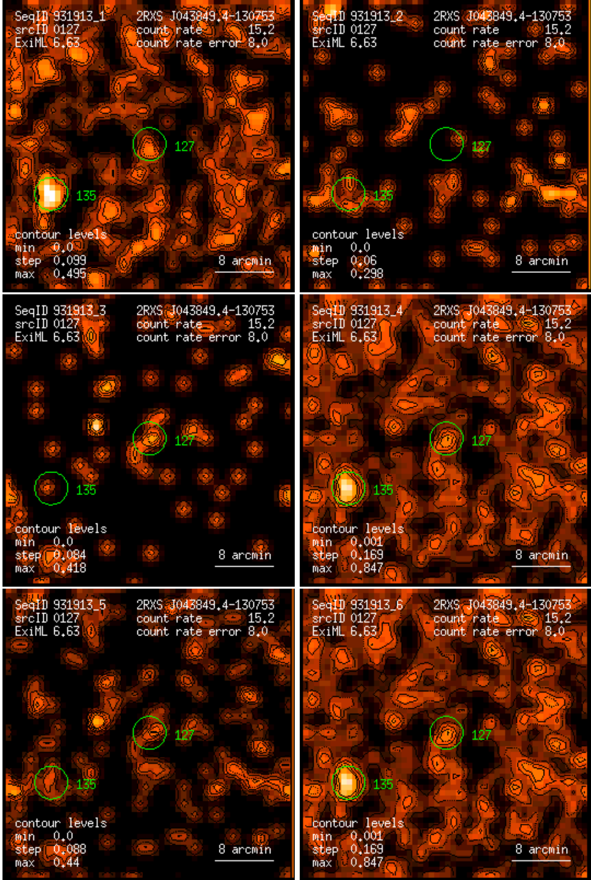
Figure 127: RASS 931913: detection 0127: band rate images, Gaussian filter: (1) PSPC channels 11 – 41, (2) 52 – 90, (3) 91 – 201, (4) 11 – 235, (5) 52 – 201, (6) 11 – 201. Broad band rates in counts/ks. Band rate contour levels in counts/ks/arcmin 2 .
