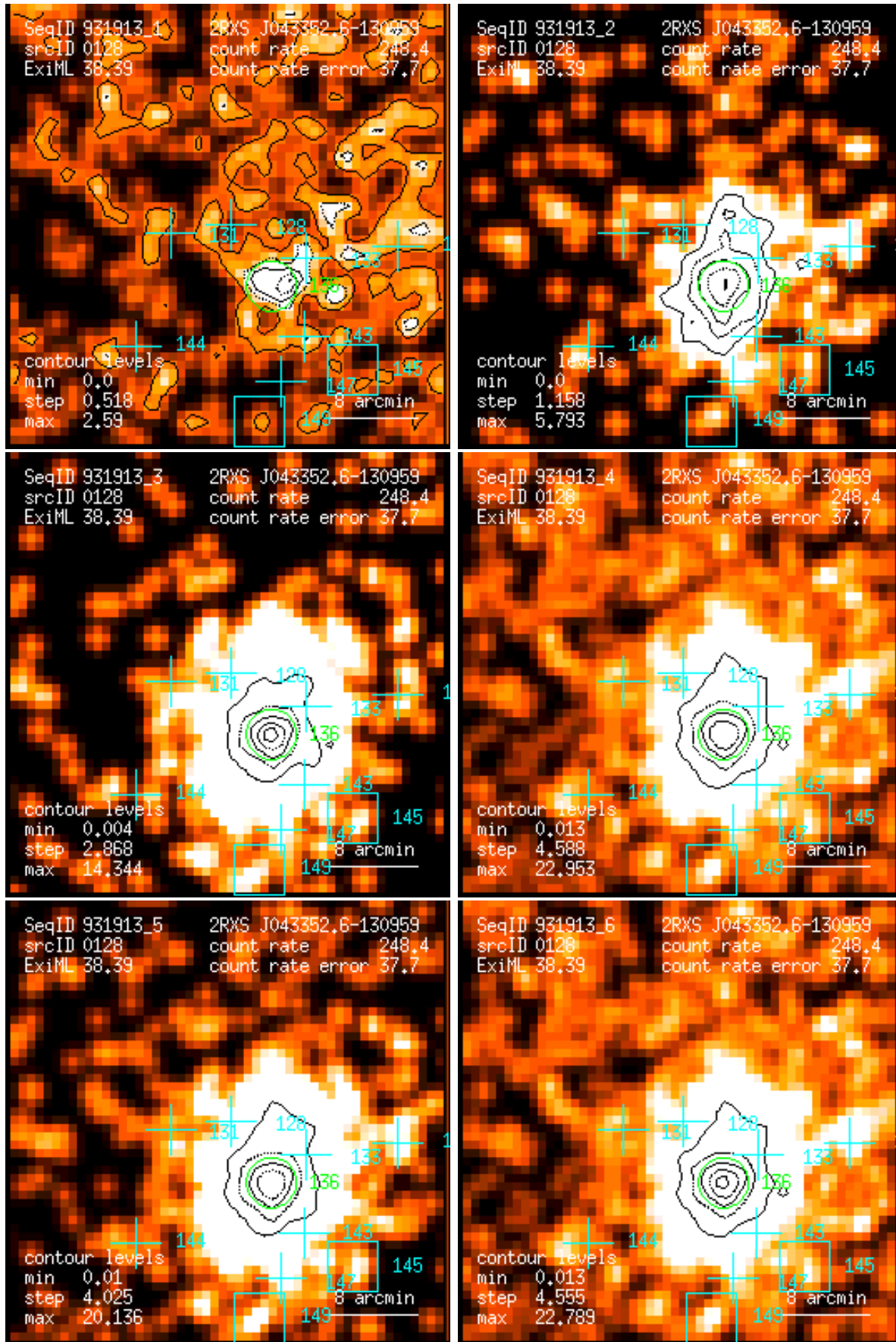
Figure 128: RASS 931913: detection 0128: band rate images, Gaussian filter: (1) PSPC channels 11 – 41, (2) 52 – 90, (3) 91 – 201, (4) 11 – 235, (5) 52 – 201, (6) 11 – 201. Broad band rates in counts/ks. Band rate contour levels in counts/ks/arcmin 2 .
