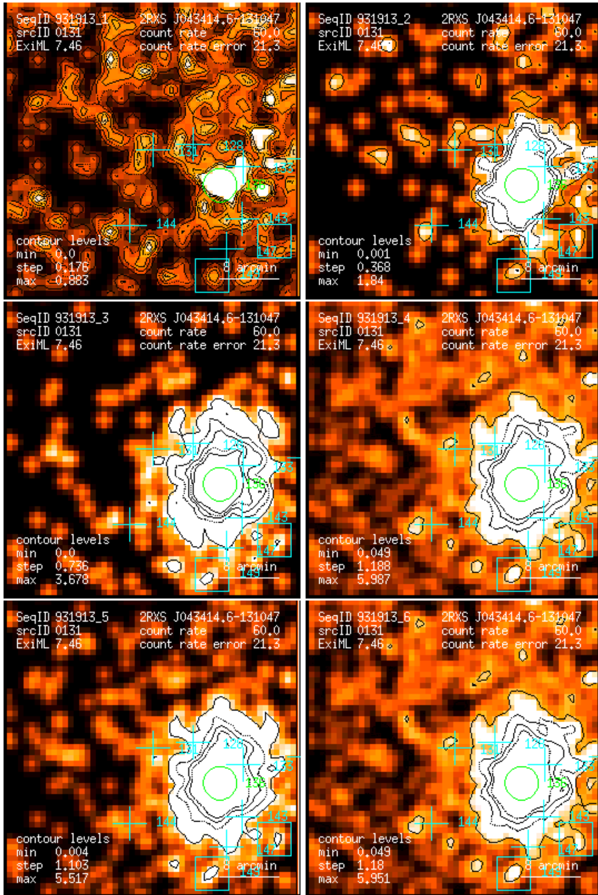
Figure 131: RASS 931913: detection 0131: band rate images, Gaussian filter: (1) PSPC channels 11 – 41, (2) 52 – 90, (3) 91 – 201, (4) 11 – 235, (5) 52 – 201, (6) 11 – 201. Broad band rates in counts/ks. Band rate contour levels in counts/ks/arcmin 2 .
