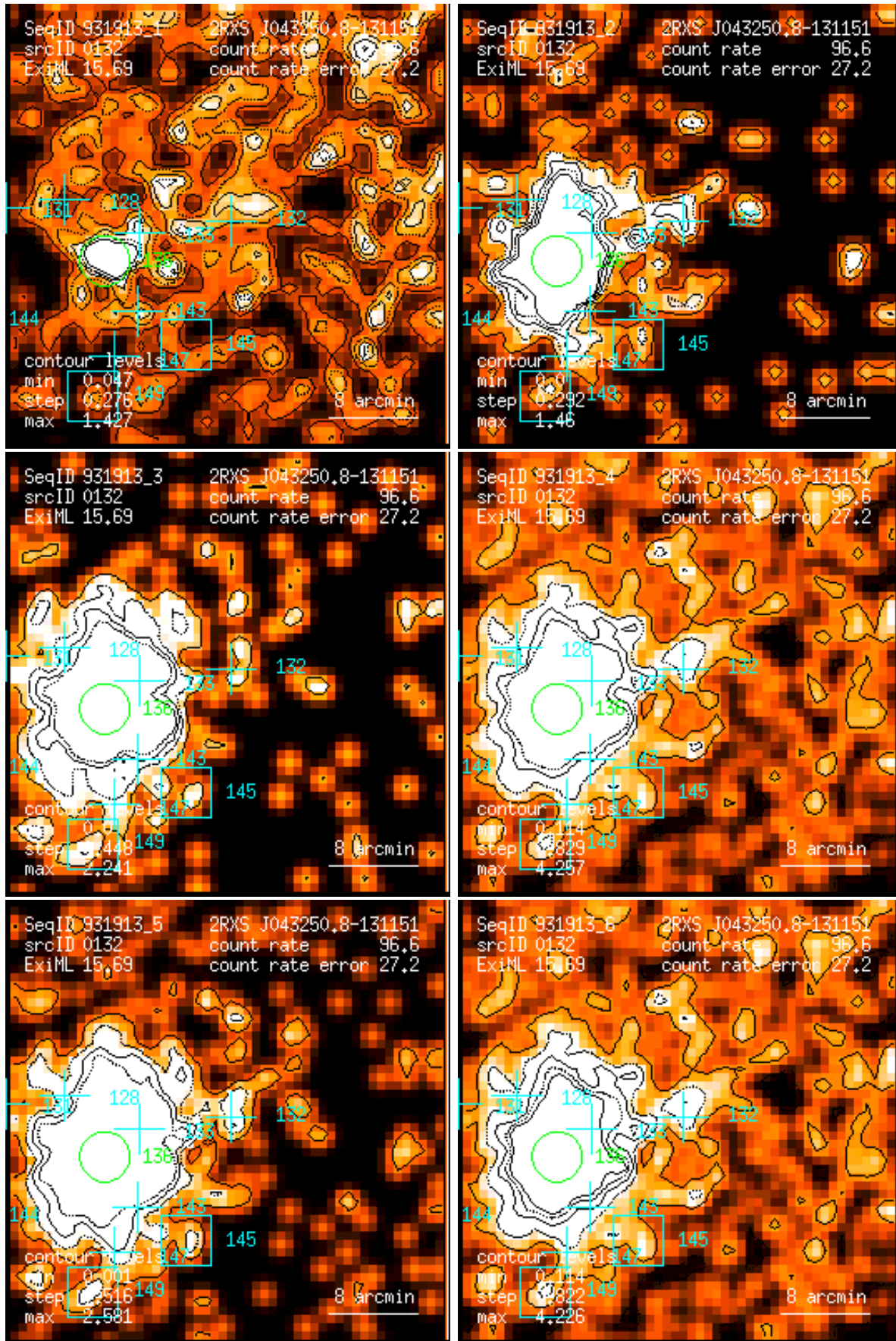
Figure 132: RASS 931913: detection 0132: band rate images, Gaussian filter: (1) PSPC channels 11 – 41, (2) 52 – 90, (3) 91 – 201, (4) 11 – 235, (5) 52 – 201, (6) 11 – 201. Broad band rates in counts/ks. Band rate contour levels in counts/ks/arcmin 2 .
