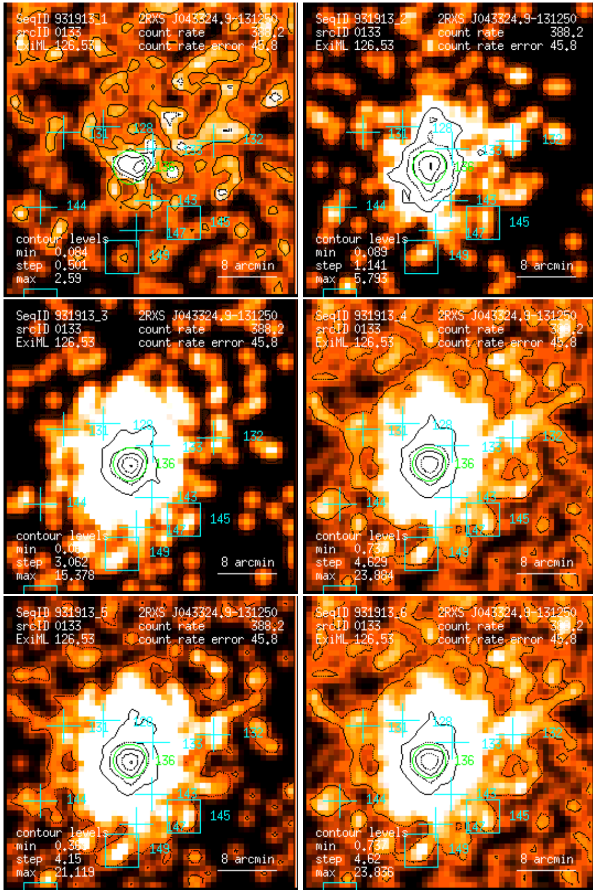
Figure 133: RASS 931913: detection 0133: band rate images, Gaussian filter: (1) PSPC channels 11 – 41, (2) 52 – 90, (3) 91 – 201, (4) 11 – 235, (5) 52 – 201, (6) 11 – 201. Broad band rates in counts/ks. Band rate contour levels in counts/ks/arcmin 2 .
