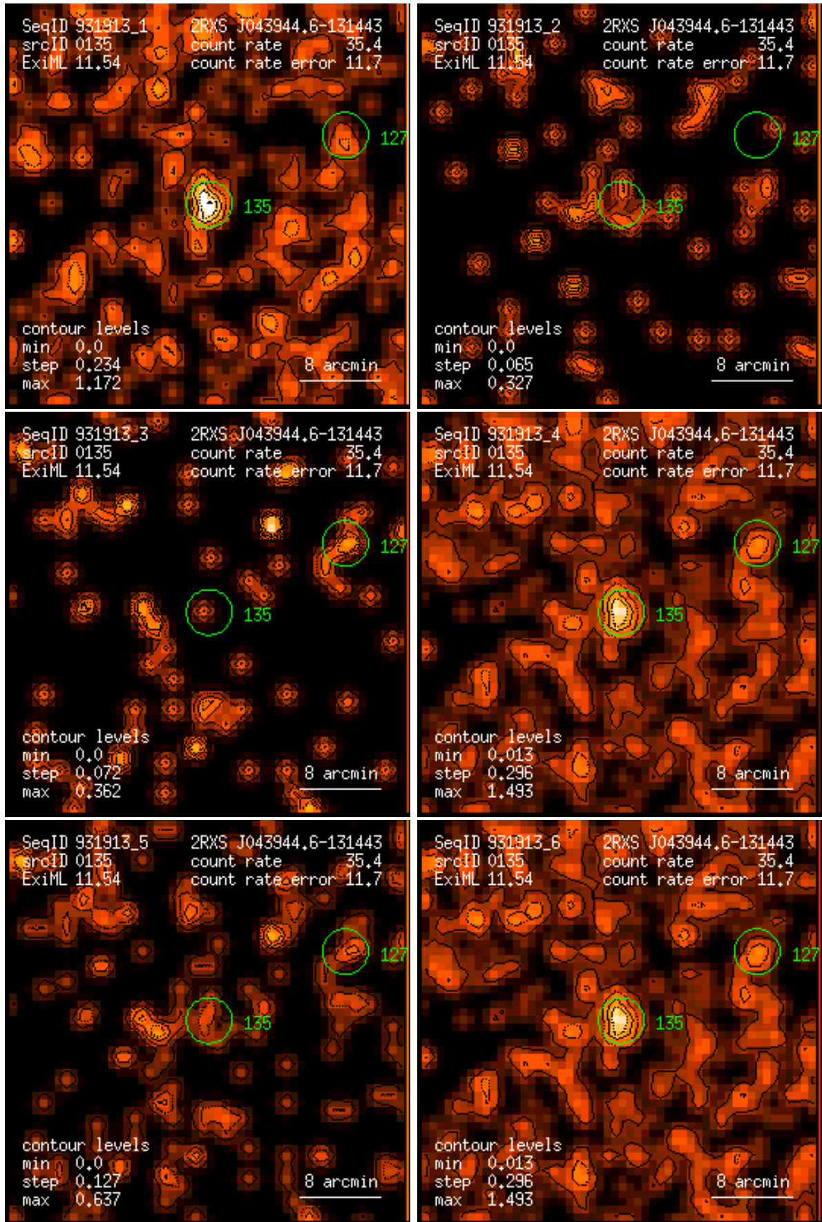
Figure 135: RASS 931913: detection 0135: band rate images, Gaussian filter: (1) PSPC channels 11 – 41, (2) 52 – 90, (3) 91 – 201, (4) 11 – 235, (5) 52 – 201, (6) 11 – 201. Broad band rates in counts/ks. Band rate contour levels in counts/ks/arcmin 2 .
