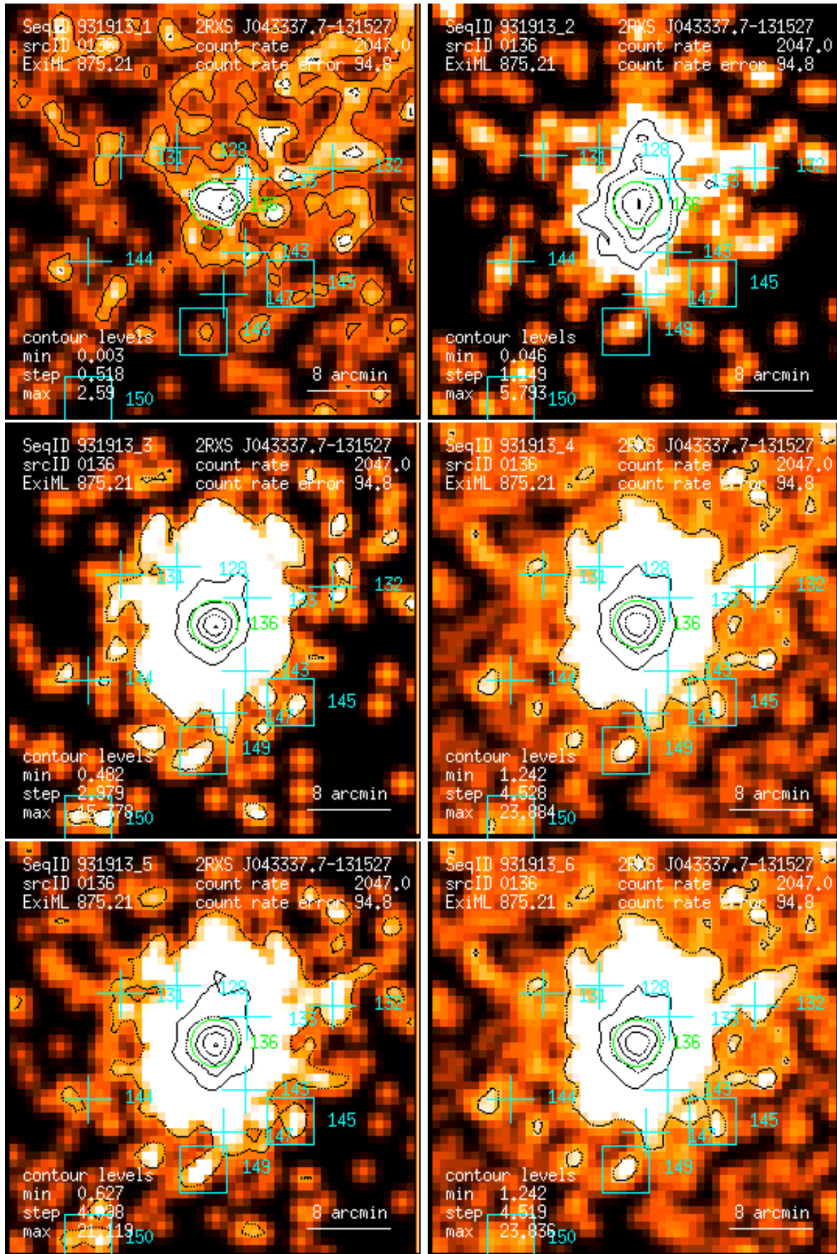
Figure 136: RASS 931913: detection 0136: band rate images, Gaussian filter: (1) PSPC channels 11 – 41, (2) 52 – 90, (3) 91 – 201, (4) 11 – 235, (5) 52 – 201, (6) 11 – 201. Broad band rates in counts/ks. Band rate contour levels in counts/ks/arcmin 2 .
