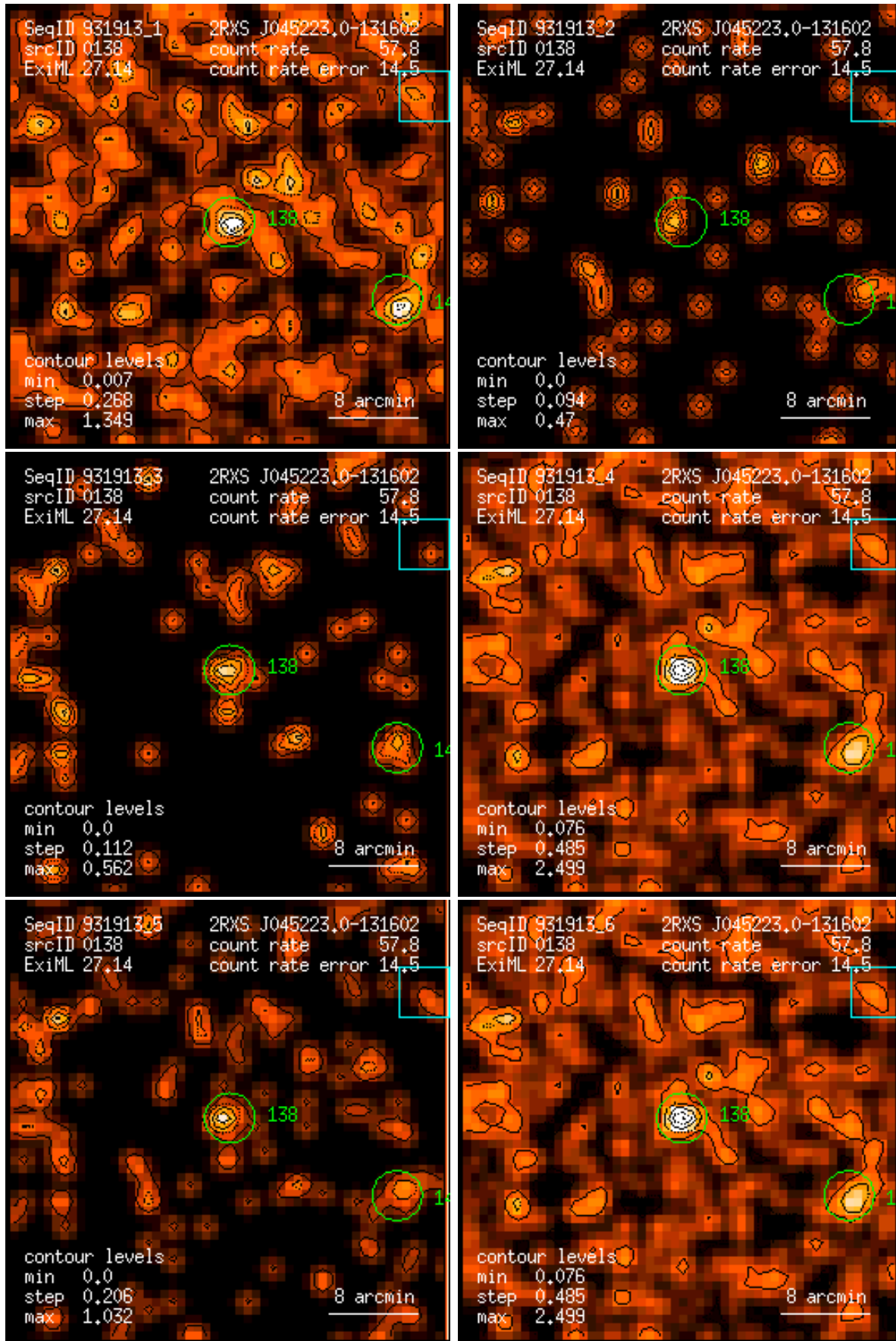
Figure 138: RASS 931913: detection 0138: band rate images, Gaussian filter: (1) PSPC channels 11 – 41, (2) 52 – 90, (3) 91 – 201, (4) 11 – 235, (5) 52 – 201, (6) 11 – 201. Broad band rates in counts/ks. Band rate contour levels in counts/ks/arcmin 2 .
